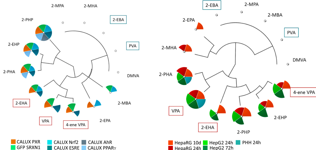
Fig. 6. Comparison of the biological activity of all analogues in the AOP relevant classes 3 (MIE and early KE in AOP) and 4 (late KE triglyceride accumulation in HepG2 cells). In vivo positive compounds (showing induction of liver steatosis primarily in preclinical rodent studies) are marked in red; in vivo negative compounds are marked in green. Minimal effect concentrations in -\log M units were normalized and hierarchical clustering was achieved using complete linkage.
