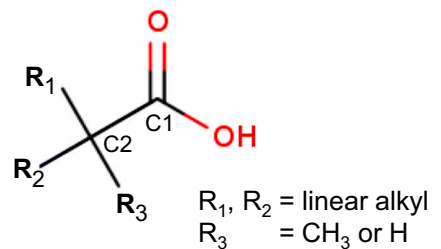
Fig. 2. Generalized chemical structure of the category members.
