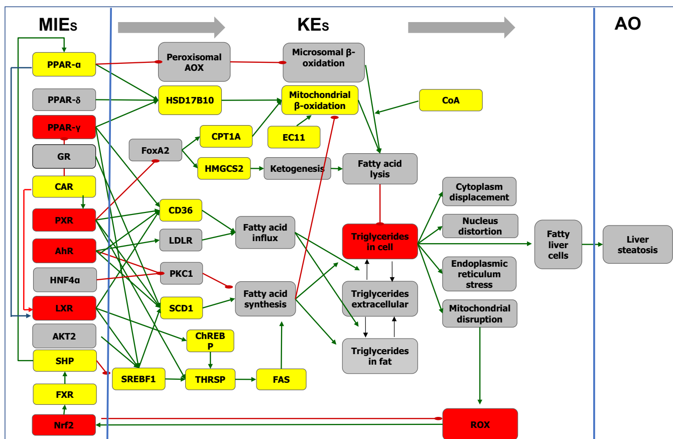
Fig. 1. The AOP network for microvesicular liver steatosis illustrates the activation and inhibition of molecular initiation events (MIEs) progressing to key events (KEs) and resulting in the adverse outcome (AO) liver steatosis; red lines indicate inhibition, green lines activation; coloured MIEs/KEs are obtained from studies testing VPA (red/yellow). Red coloured MIEs/KEs were selected for AOP specific testing in this case study. In addition endoplasmatic reticulum stress was measured. Names and abbreviations are given in Supplemental material.
