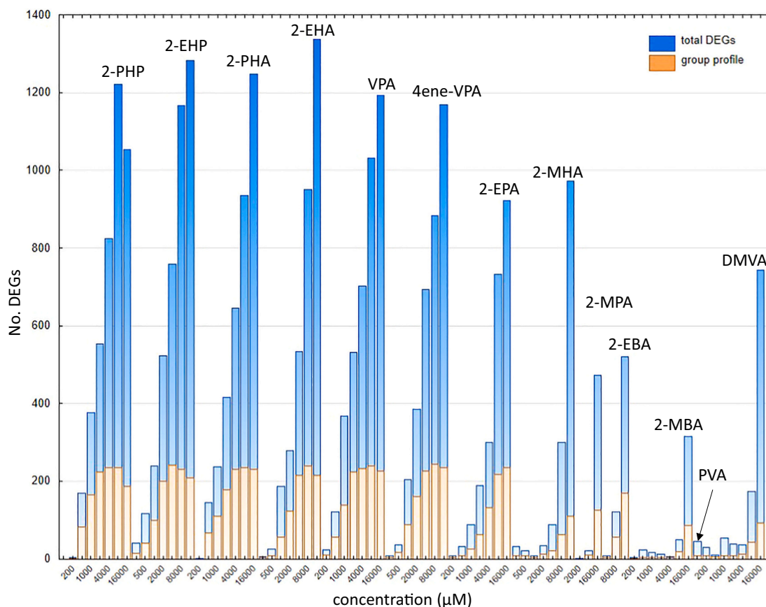
Fig. 4. Group specific DEGs – the total number of DEGs per concentration and test compound is shown (blue bars) as well as the amount of DEGs per concentration contributing to the group profile (orange bars). The majority of the shared 249 genes arise from low to moderate dose concentrations.
