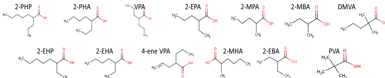
Fig. 3. Overview on case study members in order of decreasing side chain and molecular weight: 2-Propylheptanoic acid (2-PHP); 2-Ethylheptanoic acid (2-EHP); 2-Propylhexanoic acid (2-PHA); 2-Ethylhexanoic acid (2-EHA); Valproic acid (VPA); 4-ene Valproic acid (4-ene VPA); 2-Ethyl pentanoic acid (2-EPA); 2-Methyl-hexanoic acid (2-MHA); 2-Methyl-pentanoic acid (2-MPA); 2-Ethylbutyric acid (2-EBA); 2-Methylbutyric acid (2-MBA), Pivalic acid (PVA) and Dimethyl-valeric acid (DMVA).
