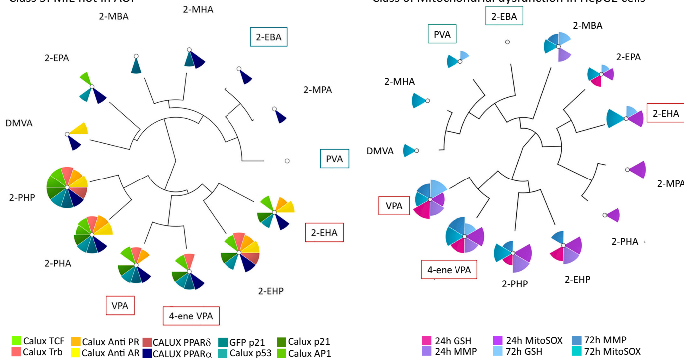
Fig. 7. Comparison of the biological activity of all analogues in the not AOP relevant classes 5 (MIE not in AOP) and 6 (Mitochondrial dysfunction in HepG2 cells). In vivo positive compounds (showing induction of liver steatosis primarily in preclinical rodent studies) are marked in red; in vivo negative compounds are marked in green. Minimal effect concentrations in -\log M units were normalized and hierarchical clustering was achieved using complete linkage.
