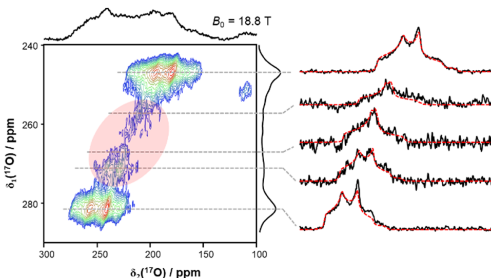
Figure 6. ^{17}\text{O} MQMAS spectrum of ZTA2a-*BDC recorded at B_0 = 18.8\text{ T} under \nu_{\text{rot}} = 16\text{ kHz} . Extracted slices (in black) are fitted (red dotted lines) with experimental parameters presented in Table 5. The red-shaded circle enlightens some of the additional oxygen sites corresponding to structural defects.
