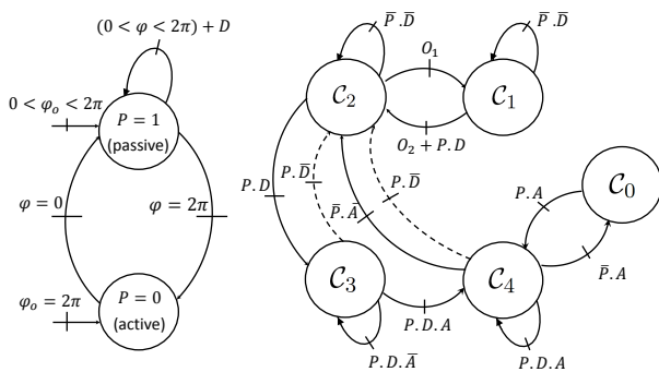
Figure 2: Graph of events of the desynchronization algorithm of aMussels and aFish (left), and of the variable structure controller of aFish navigation (right). C_{0,1,2,3,4} defines 5 reactive controllers for communication ( C_{3,4} ), obstacle avoidance ( C_{1,2} ), aggregation ( C_{3,4} ). Transitions between continuous controllers are governed by the time evolution of Boolean variables depending on the electric measurements: D means that an exogenous field is detected, P means "passive", and A "aggregated".
