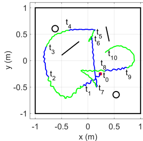
Figure 3: Paths of the aFish navigating with the controller of figure 2 in obstacle avoidance behavior C_1 (blue) and C_2 (green).
