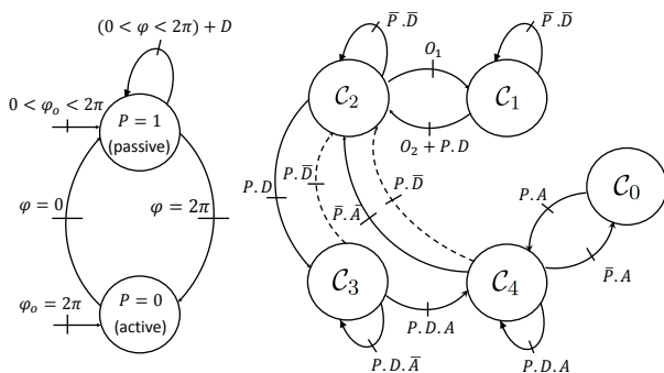
Figure 2: Graph of events of the desynchronization algorithm of aMussels and aFish (left), and of the variable structure controller of aFish navigation (right). C_{0,1,2,3,4} defines 5 reactive controllers for communication ( C_{3,4} ), obstacle avoidance ( C_{1,2} ), aggregation ( C_{3,4} ). Transitions between continuous controllers are governed by the time evolution of Boolean variables depending on the electric measurements: D means that an exogenous field is detected, P means "passive", and A "aggregated".
