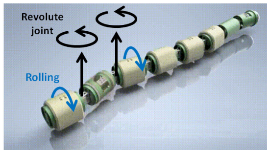
Fig. 1. The robot NATRIX with its distributed controlled rolling motions.
