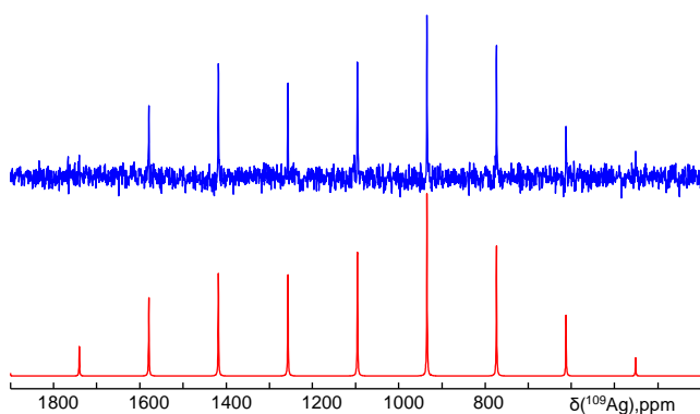
FIGURE 4. Experimental (bleu) and simulated (red), ^1\text{H} - ^{109}\text{Ag} solid state CPMAS NMR spectra of complexes [\text{Ag}_4\text{L}^a] 7 .
