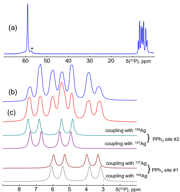
FIGURE 2. The solid state ^1\text{H}-^{31}\text{P} CPMAS NMR spectrum of the complex 6 (a). Expansion of the experimental (b) and simulated J -multiplet patterns (c) of the \text{PPh}_3 ligands. *-secondary phase.
