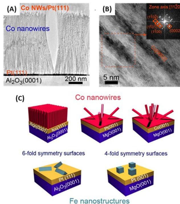
Figure 3: (A) Cross-sectional TEM micrograph of Co NW arrays grown on Pt(111)/Al 2 O 3 (0001). (B) HRTEM of (A). Inset: fast Fourier transforms illustrating the single-crystalline structure of the nanowires with a Co[0001] growth axis. (C) Schematic representation of Co NWs and Fe nanostructures directly grown on metallic films with different crystallographic orientations. Reprinted and adapted with permission from Ref. [29] Copyright 2015, American Chemical Society.
