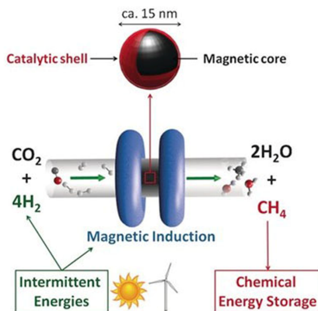
Figure 6: Schematic representation of the magnetic induced catalysis concept. Reproduced with permission from Ref. [42] Copyright 2016, Wiley-VCH.
