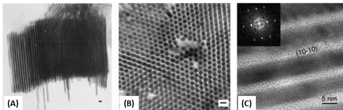
Figure 1: (A) and (B) TEM images of self-organized hcp -Co NRs (scale bars: 10 nm). (C) High Resolution TEM (HRTEM) image and electron-diffraction pattern of some aligned rods. Reprinted with permission from Ref. [23] Copyright 2003, Wiley-VCH.
