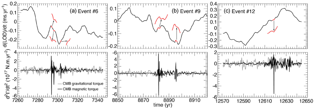
Figure 14. Top row: time-series of the length-of-day rate of change d(\text{LOD})/dt in the vicinity of jerk events 6 (a), 9 (b) and 12 (c). Bottom row: corresponding time-series of the accelerations d^2\Gamma_M/dt^2 and d^2\Gamma_G/dt^2 of the magnetic and gravitational torques, showing magnetic torque perturbations caused by jerks that significantly exceed those of the gravitational torque. The corresponding inflexions in d(\text{LOD})/dt (see eq. 5) are highlighted in red and magnified in the top row.
