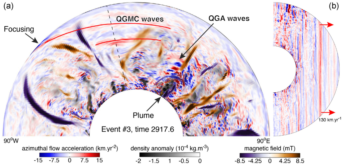
Figure 3. Structure of azimuthal flow acceleration (red/blue), density anomaly (shaded grey) and radial magnetic field (orange/purple) in a portion of the equatorial plane (a) and in a meridional plane (b) located by the dashed line in (a), during the deep wave (DW) event 3, with QGA waves being sent out by a buoyancy release at the inner core boundary (plume). The selected time is shortly before the SA pulse in the event (see Fig. 2a). The red curves in (a) locate the azimuthally elongated QGMC wave fronts.
