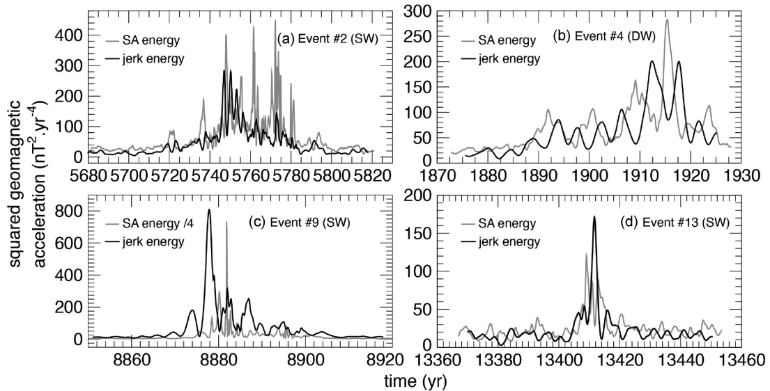
Figure 6. Time-series of the jerk energy E_J (black) and the SA energy E_{SA} (grey) during the three shallow wave (SW) events 2, 9, 13 (a,c,d) and the deep wave (DW) event 4 (b).
