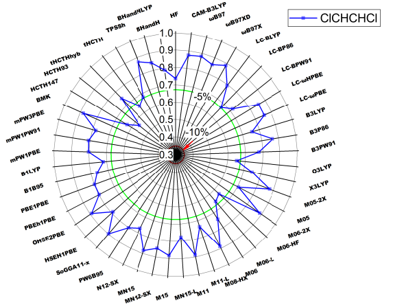
Figure 6: Similarity of calculated findings with a number of theoretical approaches towards experimental results for chloro- substituted hydrocarbons.
