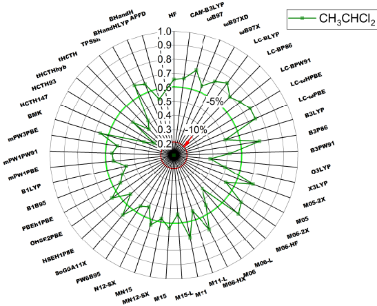
Figure 6: Similarity of calculated findings with a number of theoretical approaches towards experimental results for chloro- substituted hydrocarbons.
