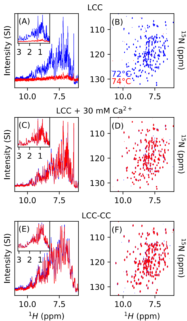
Figure 2. \text{Ca}^{2+} or the engineered disulfide bridge stabilize the enzyme beyond 74°C. (A-B) LCC without \text{Ca}^{2+} at 72°C (blue) and 74°C (red). (C-D) LCC saturated with 30 mM \text{Ca}^{2+} at 72°C (blue) and 74°C (red). (E-F) LCC-CC at 72°C (blue) and 74°C (red). (A, C, E) The main panels represent the amide region of the proton spectra, and the insets display the methyl region. (B-D-F) show ^1\text{H} - ^{15}\text{N} TROSY spectra.
