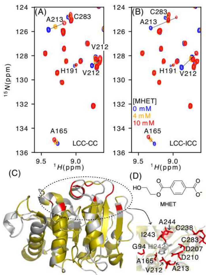
Figure 3. MHET interaction specificity at the enzyme surface. ^1\text{H} - ^{15}\text{N} TROSY spectra at 60^\circ\text{C} of LCC-CC (A), LCC-ICC (B) in absence of MHET (blue) and in the presence of 4 mM (orange) and 10 mM (red) MHET. (C) CSPs calculated from the spectra of LCC-ICC with 0 and 10 mM of MHET shown on the LCC-ICCG structure (PDB ID: 6THT). Residues for which no data are available are shown in gray, residues with 0 < \text{CSP} < 0.07\text{ppm} are shown in yellow and residue with 0.07\text{ppm} < \text{CSP} in red. The right panel indicates the residues identified with the higher CSPs surrounding the catalytic histidine H242. (D) Molecular structure of the MHET ligand.
