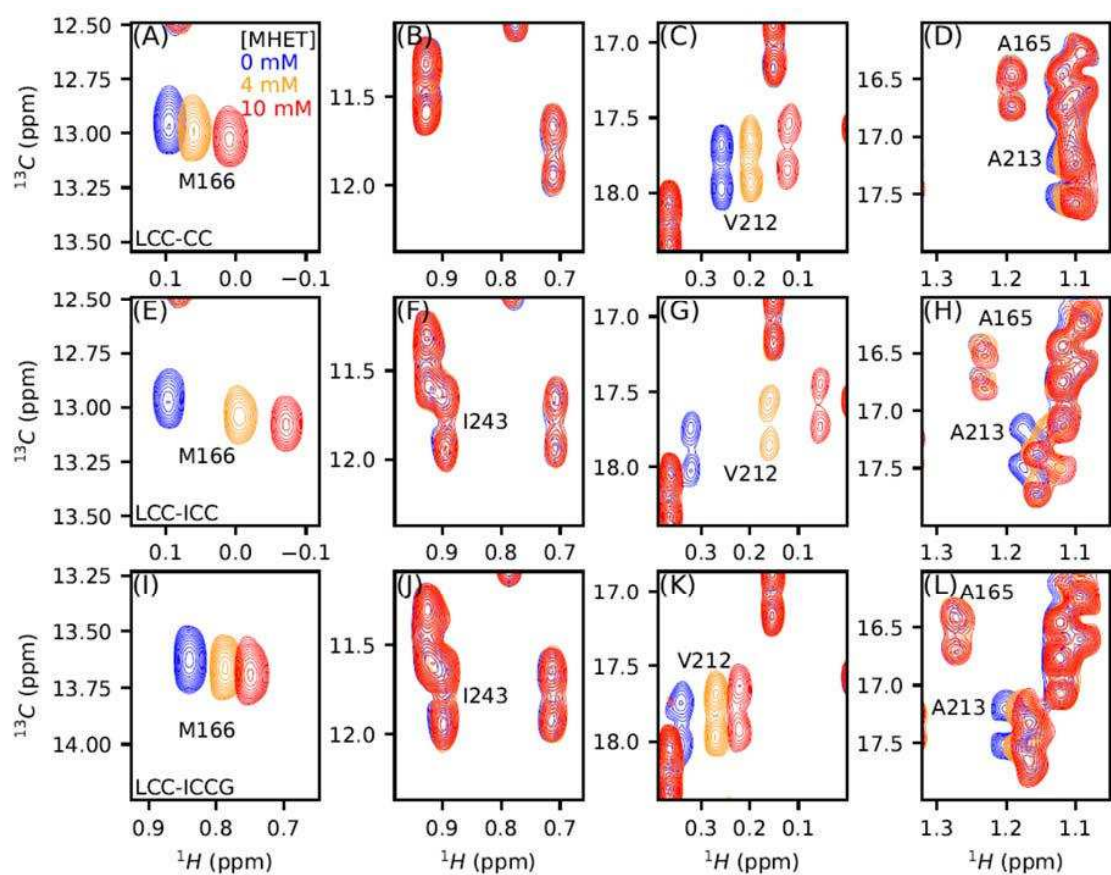
Figure 4. Methyl signals upon interaction with MHET at 60°C. Selected regions from ^1\text{H} - ^{13}\text{C} HSQC spectra of LCC-CC (A-D), LCC-ICC (E-H) and LCC-ICCG (I-L) in absence of MHET (blue) and in the presence of 4 mM (orange) and 10 mM (red) MHET.
