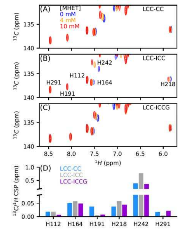
Figure 5. Histidine imidazole side chain signals upon interaction with MHET. Selected region from the ^1\text{H} - ^{13}\text{C} HMQC spectrum of LCC-CC (A), LCC-ICC (B) and LCC-ICCG (C) at 60°C in absence of MHET (blue) and in the presence of 4 mM (orange) and 10 mM (red) MHET. (D) ^1\text{H}_\epsilon - ^{13}\text{C}_\epsilon combined CSPs induced by 10mM of MHET for the histidines of LCC-CC (blue), LCC-ICC (gray) and LCC-ICCG (violet).
