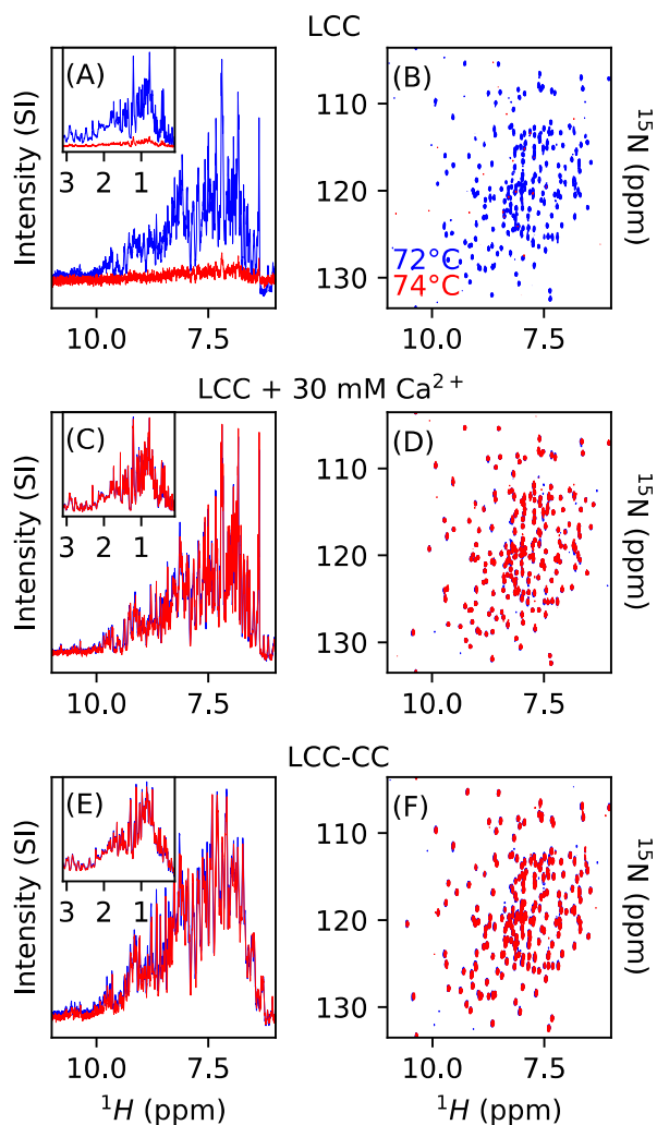
Figure 2. Ca 2+ or the engineered disulfide bridge stabilize the enzyme beyond 74°C. (A-B) LCC without Ca 2+ at 72°C (blue) and 74°C (red). (C-D) LCC saturated with 30 mM Ca 2+ at 72°C (blue) and 74°C (red). (E-F) LCC-CC at 72°C (blue) and 74°C (red). (A, C, E) The main panels represent the amide region of the proton spectra, and the insets display the methyl region. (B-D-F) show 1 H- 15 N TROSY spectra.
