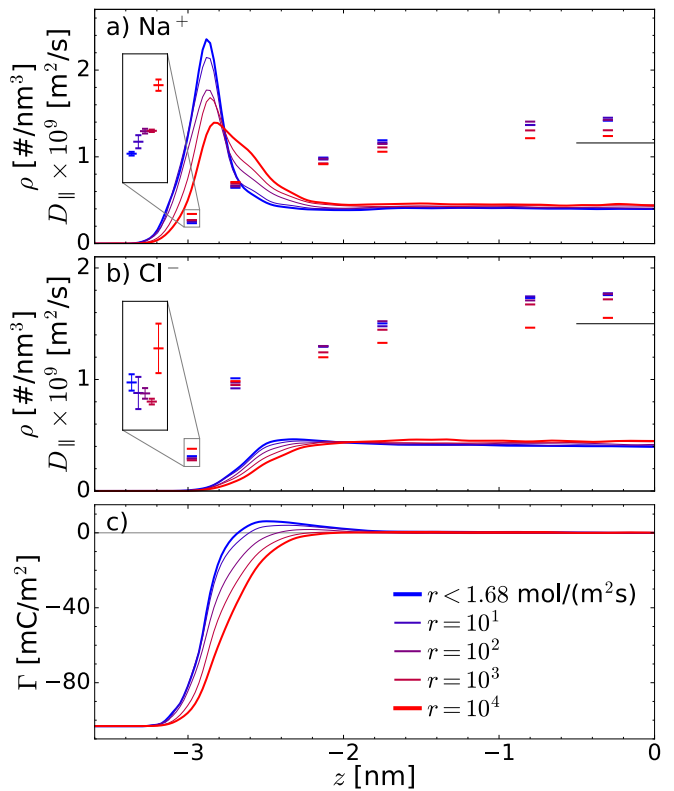
FIG. 2. a) \text{Na}^+ and b) \text{Cl}^- density profiles (lines) and parallel diffusion coefficients (symbols). Symbols in the inset are shifted in z clarity. Black lines display the bulk diffusion coefficients obtained from independent bulk electrolyte simulations (see Fig. S6 [24]). c) Screening function \Gamma . z = 0 is the channel center.
