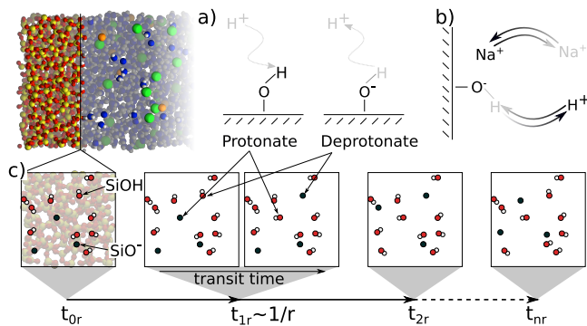
FIG. 1. a) Schematic view of protonation/deprotonation reactions at solid-liquid interfaces. Black font indicates interatomic interactions are turned on, while grey font indicates these are turned off. b) Protolysis reactions impact ion adsorption by allowing an ion to adsorb after site deprotonation (black) or forcing it to desorb after site protonation (grey). c) Simulation protocol flow diagram with time t_r \sim 1/r between protolysis reactions. Protonation/deprotonation events take place over a transit time to ensure numerical stability.
