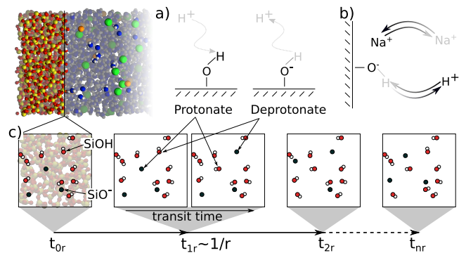
FIG. 1. a) Schematic view of protonation/deprotonation reactions at solid-liquid interfaces. Black font indicates inter-atomic interactions are turned on, while grey font indicates these are turned off. b) Protolysis reactions impact ion adsorption by allowing an ion to adsorb after site deprotonation (black) or forcing it to desorb after site protonation (grey). c) Simulation protocol flow diagram with time t_r \sim 1/r between protolysis reactions. Protonation/deprotonation events take place over a transit time to ensure numerical stability.
