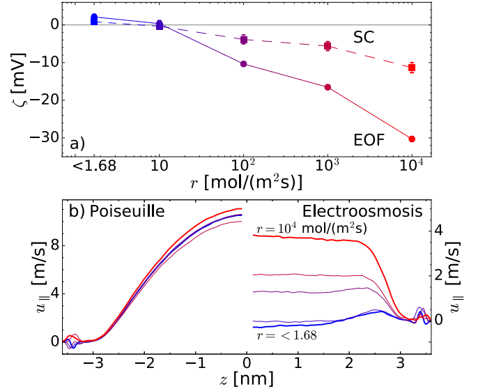
FIG. 4. a) \zeta -potential as a function of reaction rate r from streaming current (SC) and electroosmosis (EOF) simulations. b) Poiseuille (left) and electroosmosis (right) flow profiles resulting from a pressure drop of 75 atm and an electric field of 0.2 V/nm. These external forces have been shown to be within the linear response regime [28, 29].
