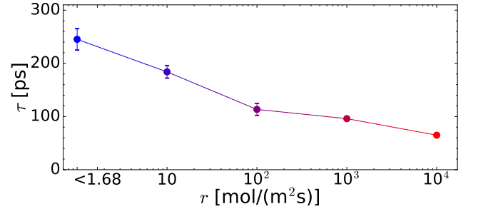
FIG. 3. Mean adsorption i.e. residence times, \tau = \int p_\tau dt (see Fig. S9 [24]) as a function of r .
