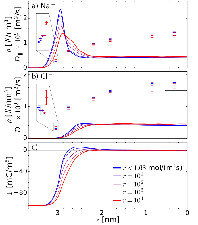
FIG. 2. a) \text{Na}^+ and b) \text{Cl}^- density profiles (lines) and parallel diffusion coefficients (symbols). Symbols in the inset are shifted in z clarity. Black lines display the bulk diffusion coefficients obtained from independent bulk electrolyte simulations (see Fig. S6 [24]). c) Screening function \Gamma . z = 0 is the channel center.
