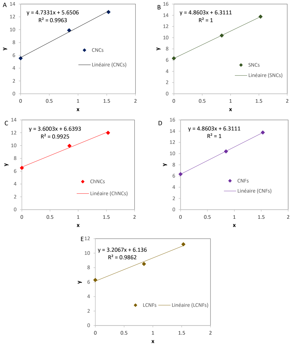
Figure S4. Plot of y = \sigma_1(\cos\theta + 1)/2 \left( \sqrt{\sigma_1^D} \right) as a function of x = \sqrt{\sigma_t^P} / \sqrt{\sigma_t^D} for the different NPs: (A) CNCs, (B) SNCs, (C) ChNCs, (D) CNFs, and (E) LCNFs.
