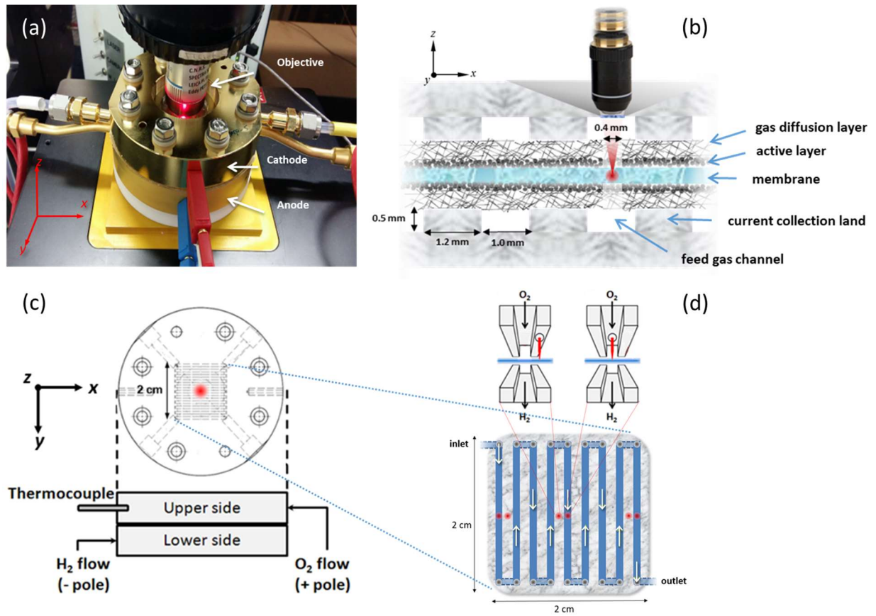
Figure 1. (a) The PEMFC for operando Raman microscopy measurements. (b) Schematic side view of the Raman probed position at the gas distribution channel. (c) Schematic top view of the bipolar plate with the carved single serpentine gas distribution channel. (d) In scale schematic representation of the configuration of the gas distribution channel and positions probed by the Raman exciting radiation.
