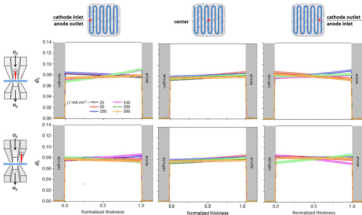
Figure 4. Comparison of the evolution of the membrane inner water distribution with the current density (reported in the legend) at the different probed positions (top: channel, bottom: lands, left: cathode inlet, middle: center, right: cathode outlet) in the cell operated at 80°C.
