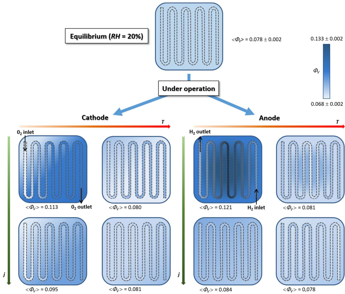
Figure 7. Schematic representation of the water distribution along the anode and cathode membrane surfaces and the effects of the FC operating T and delivered j . The positions of the gases inlet and outlet as well as of the gas distribution channels are indicated. The water content is reported as water volume fraction \Phi_V . The first scheme at the top (equilibrium) represent the homogeneous water content of the membrane in the cell at rest and spanned by H_2 and O_2 gases hydrated at 20% relative humidity.
