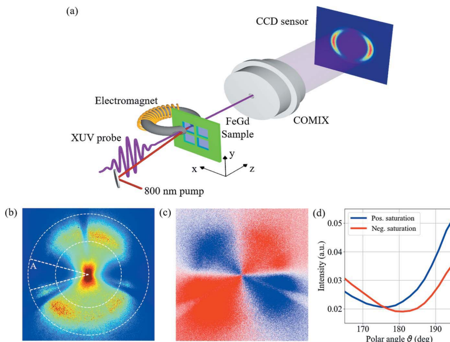
Figure 4 (a) Sketch of the experimental setup for time-resolved pump–probe measurements. (b) Intensity pattern recorded with LH polarized light tuned to 52.8 eV when the FeGd thin film was saturated along the z axis (positive saturation). (c) Difference signal between panel (b) and the corresponding image obtained saturating the sample in the opposite direction (negative saturation). By doing so, the common background can be removed, and the relative changes are highlighted. (d) Polar profiles obtained in a ±15° range around the intensity minimum labelled by A for panel (b) and for the corresponding image obtained at negative saturation. After fitting, a relative Faraday rotation of (4.6 ± 0.4)° has been evaluated.
