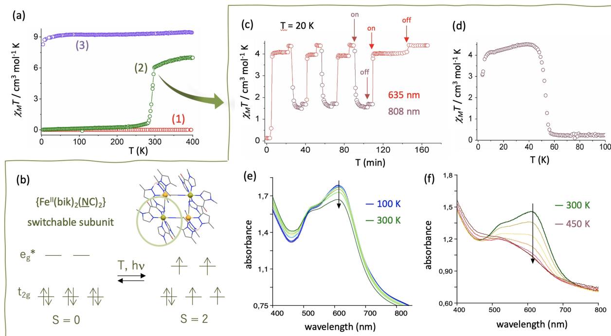
Figure 2. (a) \chi_M T versus T curves of 1–3. (b) scheme of the electronic configuration change occurring in the [\text{Fe}^{\text{II}}(\text{bik})_2(\text{NC})_2] SCO subunit in compound 2. (c) \chi_M T versus irradiation time at 635 and 808 nm in 2. Red and grey arrows indicate when the 635 and 808 lights are switched on and off. The small jump after switching off the light are due to the thermalization. (d) \chi_M T versus T curve of the photoinduced paramagnetic state ( \lambda_{\text{exc}} = 635\text{ nm} ) upon heating in darkness in 2. (e–f) Solid-state UV-vis spectra of 2 upon heating between 100 and 300 K (e) and 300–450 K (f).
