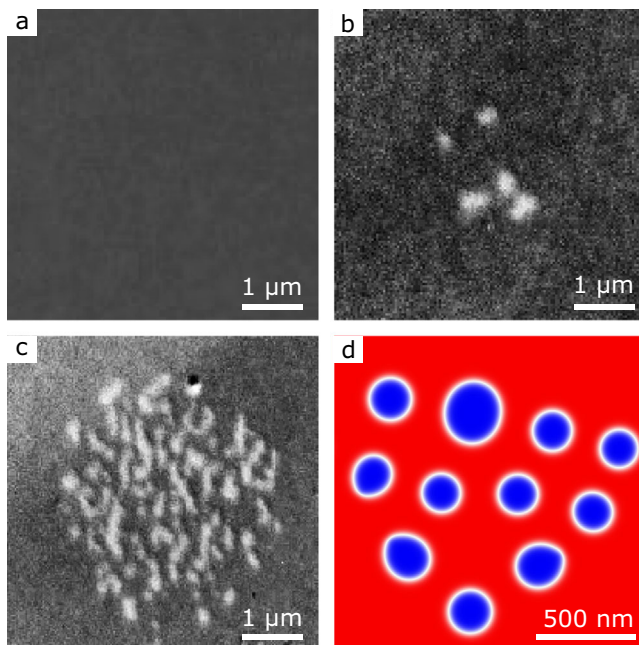
Fig. 5 | Nucleation of SAF skyrmions by ultra-fast laser pulses. a, b XMCD-PEEM images (Co L_3 edge) of a Pt(2.25)/[Pt(0.75)/Co(1.49)/Ru(0.85)] 6 (thicknesses in nanometres) SAF multilayer ( a ) before and ( b ) during the illumination of the sample by ultra-fast (80 fs) laser pulse excitation with repetition rate of 1.25 MHz and a fluence of 10 \pm 3.5 \text{ mJ cm}^{-2} in the centre of the beam ( c ) XMCD-PEEM image of worm domains and skyrmions after the continuous illumination (several minutes) by ultra-fast laser pulses with a fluence of 7.0 \pm 2.5 \text{ mJ cm}^{-2} . The experiments were carried out at zero field. d Micromagnetic simulation using experimental parameters. Magnetisation distribution ( m_z in colour scale (cf Fig. 2a) obtained after relaxation from a random initial state, mimicking a fully demagnetised state resulting from the laser excitation. Scale bars in a, b, c, d are 1 \mu\text{m} and 500 nm, respectively.
