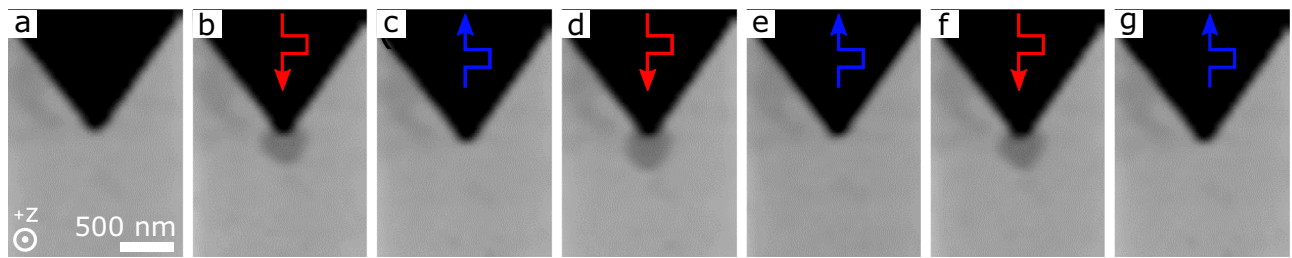
Fig. 4 | Current-induced nucleation/annihilation of SAF skyrmions.
