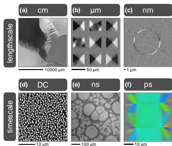
Figure 1. Exemplary Kerr microscopy images on different length and time scales. (a) Large view domain image from a mixed low anisotropy \text{Ni}_{81}\text{Fe}_{19} (40 nm) single film. (b) Variations from Landau domain structures in \text{Ni}_{81}\text{Fe}_{19} (50 nm) square elements. (c) Magnetic onion state in a 300 nm width \text{Co}_{90}\text{Fe}_{10} (0.8 nm)/ \text{Ni}_{81}\text{Fe}_{19} (28 nm) ring structure [1]. (d) Quasi-static domain image of skyrmion bubble formation in a \text{Co}_{40}\text{Fe}_{40}\text{B}_{20} (1.4 nm)/MgO thin film. (e) Single-shot dynamic domain evolution in a micrometre thick garnet layer (single shot imaging with 20 ns pulse width, MO Faraday contrast imaging). (f) Quantitative dynamic domain imaging of spin waves in a \text{Co}_{40}\text{Fe}_{40}\text{B}_{20} (120 nm) film (excitation frequency of 3 GHz, time resolution of 7 ps) [6].
