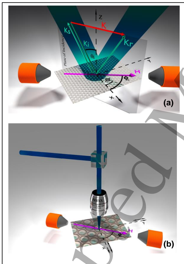
Figure 1. (a) Scattering geometry of the conventional BLS experiment in the so-called back-scattering configuration. The wave vector of the incident, reflected and scattered light is indicated, together with the in-plane direction of the applied magnetic field. The illuminated area of the sample has a typical diameter of 30-40 microns (b) Schematic drawing of the micro-BLS apparatus, where BLS is operated as a scanning-probe technique. The illuminated area of the sample has a typical diameter of 0.25-0.30 microns.
