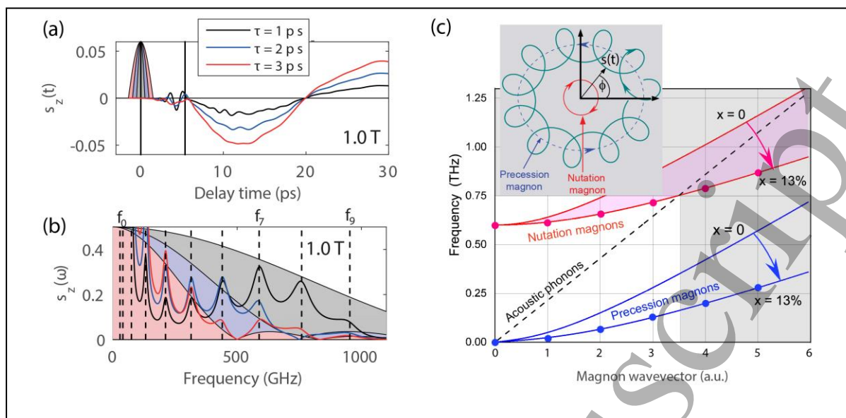
Figure 2. (a) Ultrafast magnetization dynamics driven by a single acoustic pulse traversing through a 30 nm thin layer of ferromagnetic Nickel shows that (b) nearly all exchange magnon modes within the acoustic bandwidth can be excited. Dashed colored areas in (a) and (b) show temporal profiles and Fourier spectra of three distinct acoustic pulses with 1, 2, and 3 picosecond time duration, respectively [10]. (c) When experimentally accessible, THz-frequency magneto-elastic interaction spectroscopy could be used to quantify the phenomenon of the inertial magnetization dynamics [6,7], which should manifest itself in the appearance of an upper (THz)-frequency band of nutation magnons [8]. Simulation performed for Gd-doped Permalloy thin films \text{Gd}_x\text{Py}_{1-x} , characterized through \sim 10 GHz-frequency time-domain exchange magnon spectroscopy [2]. The inset shows an exemplary flower-like magnetization trajectory consisting of two magnon modes from different branches, which are precessing in opposite directions. Fig. 2(a,b) adapted with permission from Ref. [10]; Fig. 2(c) adopted with permission from Ref. [8].
