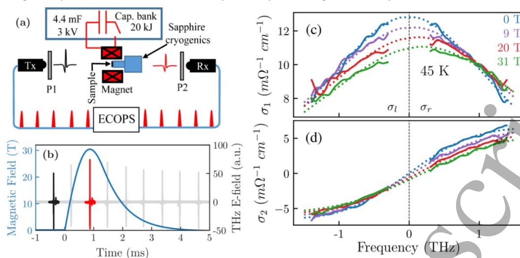
Figure 2. (a) Experimental schematic. A small pulsed magnet is incorporated with an ECOPS-based TDS system. Broadband THz optical pulses generated by the transmitter (Tx) are linearly polarized (by P1) and focused through the sample in the magnet and directed through a second polarizer (P2) and detected by the gated receiver (Rx). Parabolic collimating and focusing mirrors not shown. (b) The field profile of a 31 T magnet pulse (blue, left axis) is plotted along with the simultaneously measured THz electric field (right axis). (c) and (d) Experimentally measured optical conductivity from LSCO up to 31 T at 45 K. A clear cyclotron shift is observed, along with and broadening consistent with increasing scattering rate. Dashed lines show fits using a cyclotron model. From Ref. [7].
