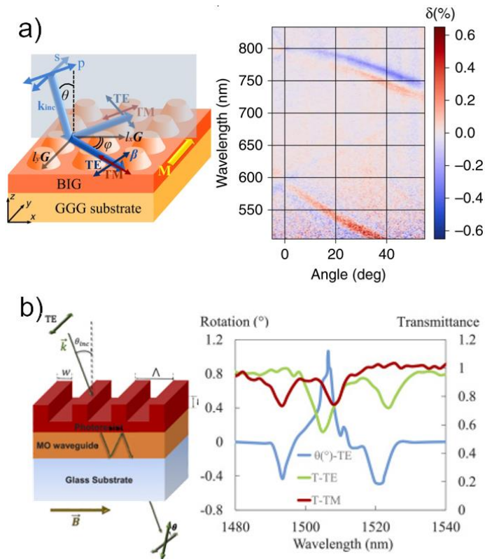
Figure 1. Unusual magneto-optical response of all-dielectric magneto-optical metasurfaces. a) Transverse magnetophotonic intensity effect observed in s-polarized light in 2D metasurface. This effect equals to zero for an unstructured smooth magnetic film. [4]. b) Significant enhancement of longitudinal magneto-optical effect at 0.4 deg angle of incidence [5]. This effect is several orders lower for a same smooth magnetic film.
