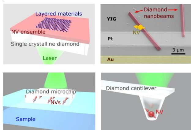
Figure 2. NV centers contained in a single crystalline diamond, diamond nanobeam, diamond microchip, and diamond cantilever for quantum sensing measurements. The top right panel is taken from Ref. 4.
