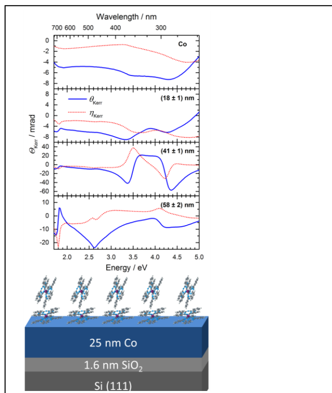
Figure 1. MOKE spectra of a Co film (top) and of thin films of the single molecule magnet TbPC 2 on Co/SiO 2 /Si recorded at room temperature in the paramagnetic state. The TbPC 2 film thickness is given in the legend of each graph. The continuous lines (blue) and dotted lines (red) represent the spectra of the Kerr rotation and ellipticity, respectively. (bottom) Sketch of the samples. Reproduced from Ref. [5] with permission from the Royal Society of Chemistry.
