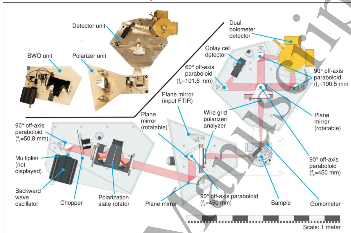
Figure 1. THz-EPR-E instrumentation adapted from an optical Hall effect instrumentation at the Terahertz Materials Analysis Center, Lund University. (Top left) Photograph (top view). (Bottom right) To scale drawing of all optical components. Future designs envision use of all-solid-state synthesizer THz source and detector components. Reprinted with permission from [13]. Copyright 2018 Institute of Electrical and Electronics Engineers.
