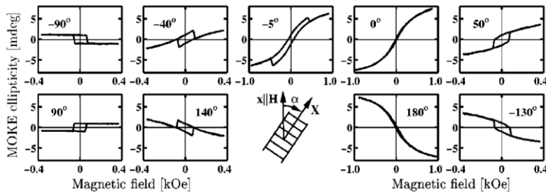
Figure 2. Magnetization loops of MOKE on vicinal structure Co/Au(322) at different sample orientations with in-plane applied field. The measured MOKE consists of vicinal MOKE, originating from a higher order term \varepsilon_{yz\varepsilon_{zx}} [7]. The vicinal MOKE is linear in magnetization, however remarkably changes sign when sample is rotated by 180 deg.
