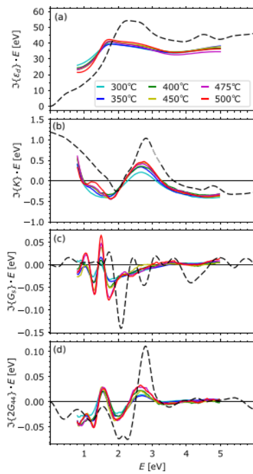
Figure 1. Imaginary part of permittivity spectra of Heusler compound \text{Co}_2\text{MnSi} prepared at different annealing temperatures, corresponding to different amount of L2_1 ordering (a) \epsilon_d (permittivity of zeroth order in M ), (b) linear MO parameter K , (c) quadratic MO parameter G_s , and (d) quadratic MO parameter 2G_{44} . Colored full lines are the experimental spectra, black dashed lines are ab initio spectra [5].
