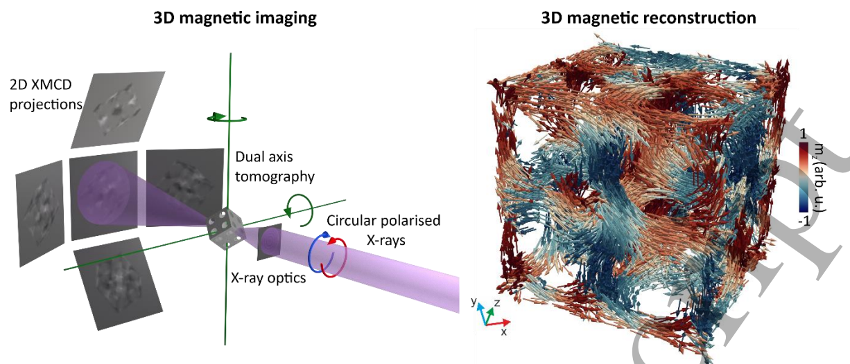
Figure 1. 3D X-ray magnetic imaging requires the measurement of XMCD projections for a number of different orientations of the sample. These projections are then combined using a reconstruction algorithm to obtain a map of the magnetisation vector field.
