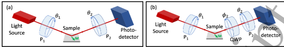
Figure 1. Schematic arrangements of experimental GME setups that have been utilized, namely (a) the conventional GME setup and (b) the more recently explored T-MOKE ellipsometry configuration; both detection schemes utilize a light source, which is a laser in most realizations, a linear polarizer P_1 in the incoming beam, a second linear polarizer P_2 in the reflected beam and a photodetector. The T-MOKE ellipsometry system in (b) furthermore contains a quarter wave plate QWP. In both approaches, a magnetic field sequence is applied to the sample to produce inverted magnetization states, whose signal difference at the photodetector is recorded for a sequence of optical element alignments. In (a), a series of polarization angle pair settings (\theta_1, \theta_2) for P_1 and P_2 is explored, while the methodology in (b) relies on a series of angle pair settings (\phi_2, \theta_2) for QWP and P_2 .
