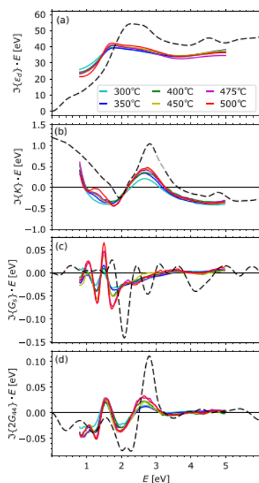
Figure 1. Imaginary part of permittivity spectra of Heusler compound \text{Co}_2\text{MnSi} prepared at different annealing temperatures, corresponding to different amount of \text{L}_{21} ordering (a) \varepsilon_d (permittivity of zeroth order in M ), (b) linear MO parameter K , (c) quadratic MO parameter G_s , and (d) quadratic MO parameter 2G_{44} . Colored full lines are the experimental spectra, black dashed lines are ab initio spectra [5].
