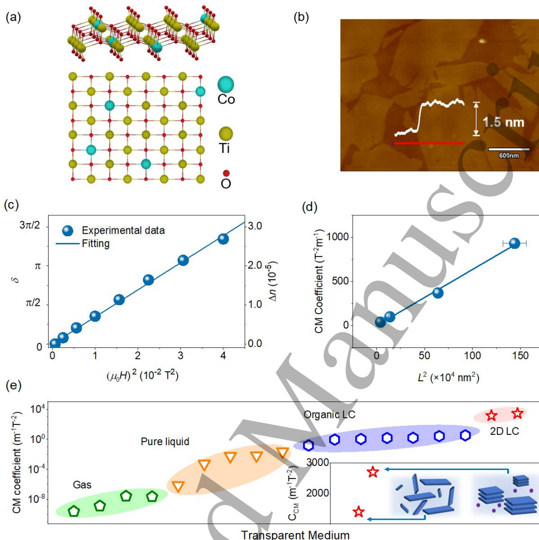
Figure 2. Giant magneto-optical Cotton-Mouton effect of 2D cobalt doped \text{TiO}_2 (CTO). (a) Atomic structure of 2D CTO. (b) AFM image of 2D CTO. (c) Magnetic-field dependence of the birefringence in the low-field range for 2D CTO LC. Symbols: experimental data; solid line: linear fit. Here, birefringence is proportional to the square of magnetic field. (a) – (c) are adapted by permission from Springer Nature Ltd: Nature Communications [2], Copyright 2020. (d) CM coefficient verse L^2 ( L is the lateral size). The fitting result gives that the CM coefficient has a linear dependence with the square of lateral size of 2D CTO. Adapted with permission from [12]. Copyright 2021 American Chemical Society. (e) Summary of the CM coefficient obtained so far among all transparent media, including gas, pure solvent, organic LC and 2D CTO LC. Inset shows the comparison of CM coefficient between collective-behavior dominant and individual-behavior dominant 2D CTO LC. Adapted with permission from [14]. Copyright 2021. American Chemical Society. Adapted with permission from [14]. Copyright 2021 American Chemical Society.
