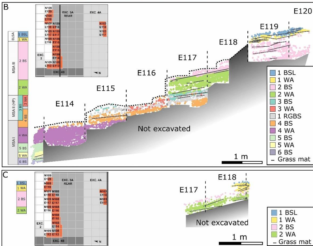
Fig. 2. A , Photograph of excavations conducted from 2015 to 2019 along the North face of Beaumont’s excavation (EXC.) 3A trench. The youngest deposits are towards the back of the cave on the right, and the oldest towards the centre of the cave on the left. B , Stratigraphic sequence along the North wall with plotted grass mats/bedding shown as dipping horizontal black lines. The dashed line indicates the bottom limit of Beaumont’s excavations. C , Stratigraphic sequence along the South wall with grass mats/bedding shown as black lines. The
