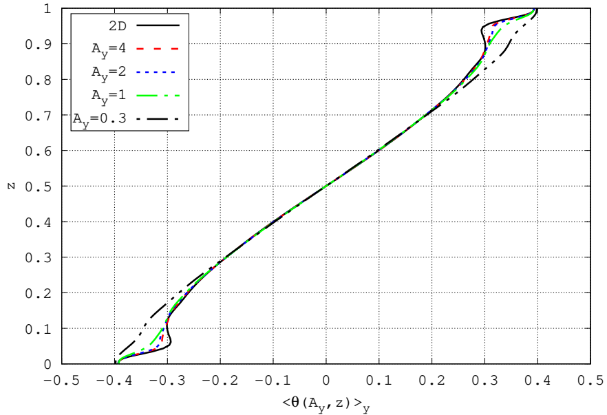
FIG. 7: For various horizontal aspect ratios A_y (0.3, 1, 2, 4), vertical profile of the y-averaged temperature \langle \theta(A_y, z) \rangle_y in the mid-width plane x = \frac{A_y}{2} versus the cavity height z . The two-dimensional case is also presented for comparison.
