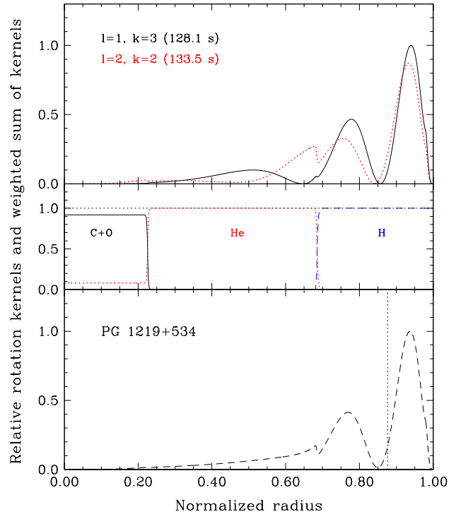
Figure 8. Top panel: Relative rotational kernels K_{kl} as a function of normalized radius for the two multiplet structures associated to 128.1 s and 133.5 s periods observed in the light curve of PG1219+534. Middle panel: Chemical stratification of the model. Bottom panel: Weighted sum of the kernels versus normalized radius. The vertical dotted line defines the layer where half of the running integral of the weighted sum is below and the other half above.
