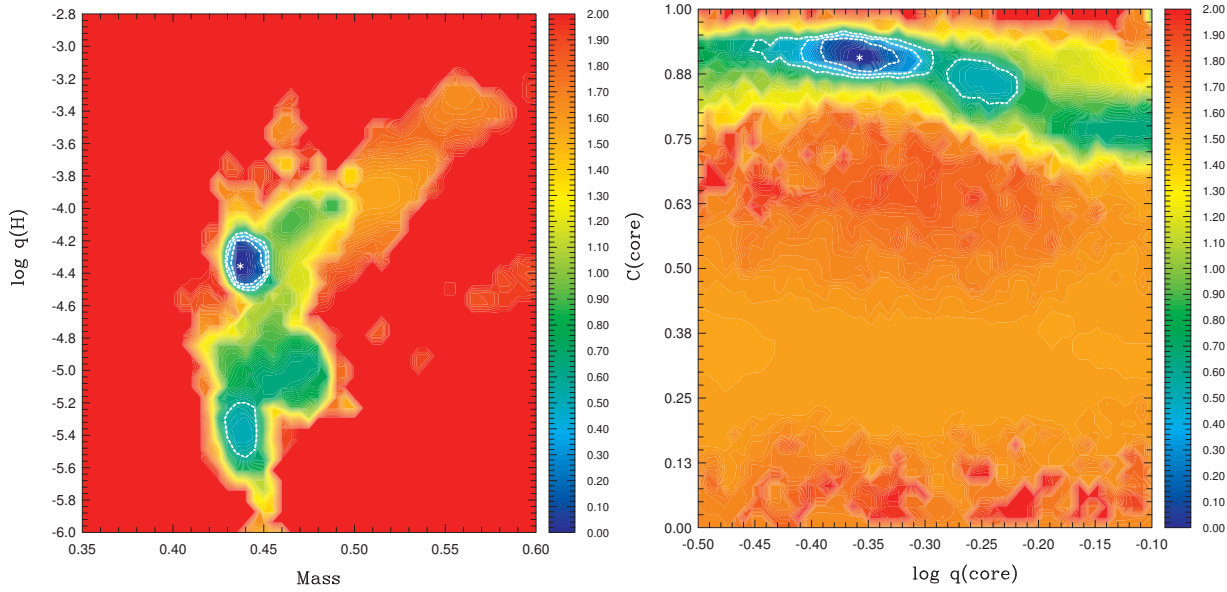
Figure 5. Optimization with 3G models. Left panel: Map of the projected merit function S^2 (on a logarithmic scale) in the \log q(\text{envl})-M_* plane. At each M_* , \log q(\text{envl}) position, the value given is the minimum of \log S^2 that can be found among the values obtained for all \log q(\text{core}) and X_{\text{core}}(C + O) . Right panel: Map of the projected merit function S^2 (on a logarithmic scale) in the \log q(\text{core})-X_{\text{core}}(C + O) plane where the best-fit model is indicated by a star. White contours show regions where the period fits have S^2 values within the 1\sigma , 2\sigma and 3\sigma confidence levels relative to the best-fit solution.
