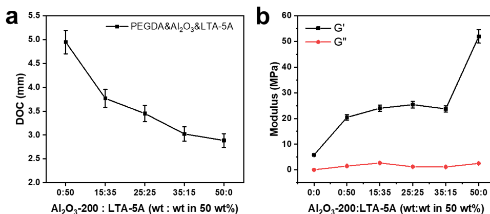
Fig. 2. (a) DOC and (b) DMA for two fillers-based composites with different [Al 2 O 3 -200] : [LTA-5A] ratios.
