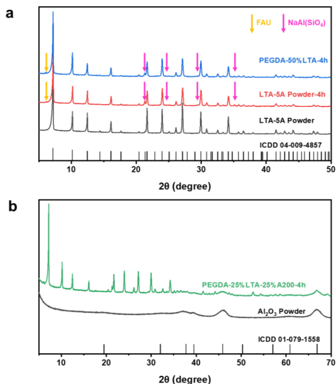
Fig. 7. XRD for (a) LTA-5A powder, LTA-5A powder-4h and PEGDA-50%LTA-4h; (b) Al 2 O 3 powder and PEGDA-25%LTA-25%A200-4h.
