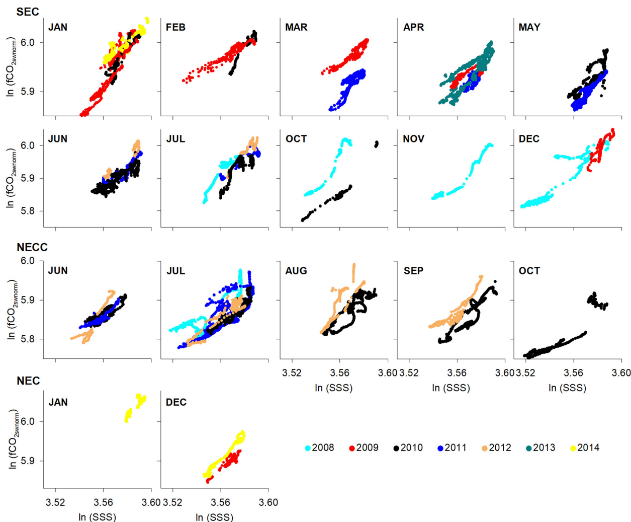
Fig. 4. \ln f\text{CO}_{2\text{swnorm}} vs \ln \text{SSS} constructed with the underway data with interpolated, short-term rainfall higher than 1 mm, discriminated by surface current (SEC, NECC, NEC) and month. Color code shown in the figure legend is used to indicate year. During January 2009, June 2010, July 2011 and April 2013, significant linear relationships of \ln f\text{CO}_{2\text{swnorm}} vs \ln \text{SSS} were found in the northbound and southbound voyages.
