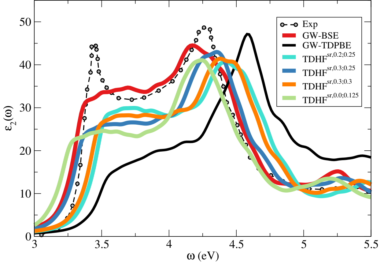
FIG. 4. Comparison of experimental \epsilon_2 for Si with GW-BSE, GW-TDPBE, \text{TDHF}^{sr,0.2;0.25} , \text{TDHF}^{sr,0.3;0.25} , \text{TDHF}^{sr,0.3;0.3} and \text{TDHF}^{sr,0.0;0.125} and PAW pseudopotential. Experiment is from Ref. [46].
