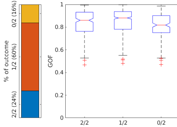
Fig. 1. Ambiguity results. Left panel, the proportion of different outcomes (in blue (24%): both alternative sources were among the 3 simulated ones; in red (60%): one of the sources was far from the simulated ones; in yellow (16%): both alternative sources were far from the simulated ones. Right panel, the GOF of the reconstructed signal \hat{\mathbf{X}} with respect to the original \mathbf{X} for the three possible outcomes in the left panel.
