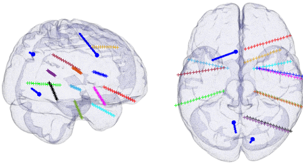
Fig. 2. Three sources placement in the brain. They are illustrated in blue arrows representing positions and orientations of sources. Electrodes are represented as crosses and each one with a different color. For illustrative purposes, source amplitudes are shown 40% larger of their original.
