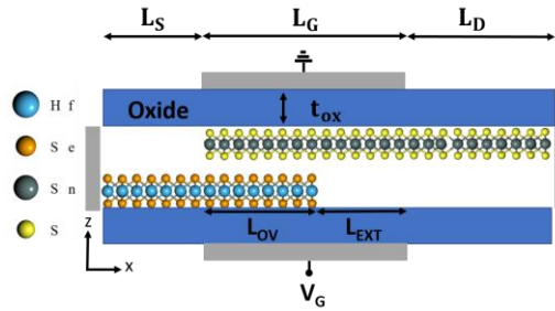
Figure 1. VdW TFET sketch with L_{S/D}=8\text{nm} , L_G=15\text{nm} , L_{OV}=10\text{nm} , L_{EXT}=5\text{nm} .
