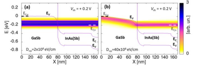
Fig. 11. Current spectra as in Fig. 10 but here for V_{\text{ds}} = +0.2 V.
