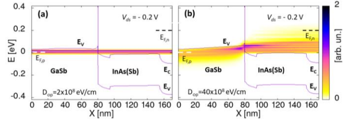
Fig. 10. Current spectra for the simulations in Fig. 9 (b) at V_{\text{ds}} = -0.2 V. (a): D_{\text{op}} = 2 \times 10^8 eV/cm and (b): D_{\text{op}} = 40 \times 10^8 eV/cm. The energy reference is the Fermi level ( E_{f,p} ) in GaSb, so that E_{f,n} on the InAs side is given by -qV_{\text{ds}} . The lines refer to the spatial profiles of the highest valence subband ( E_v ) and of the lowest conduction subband ( E_c ).
