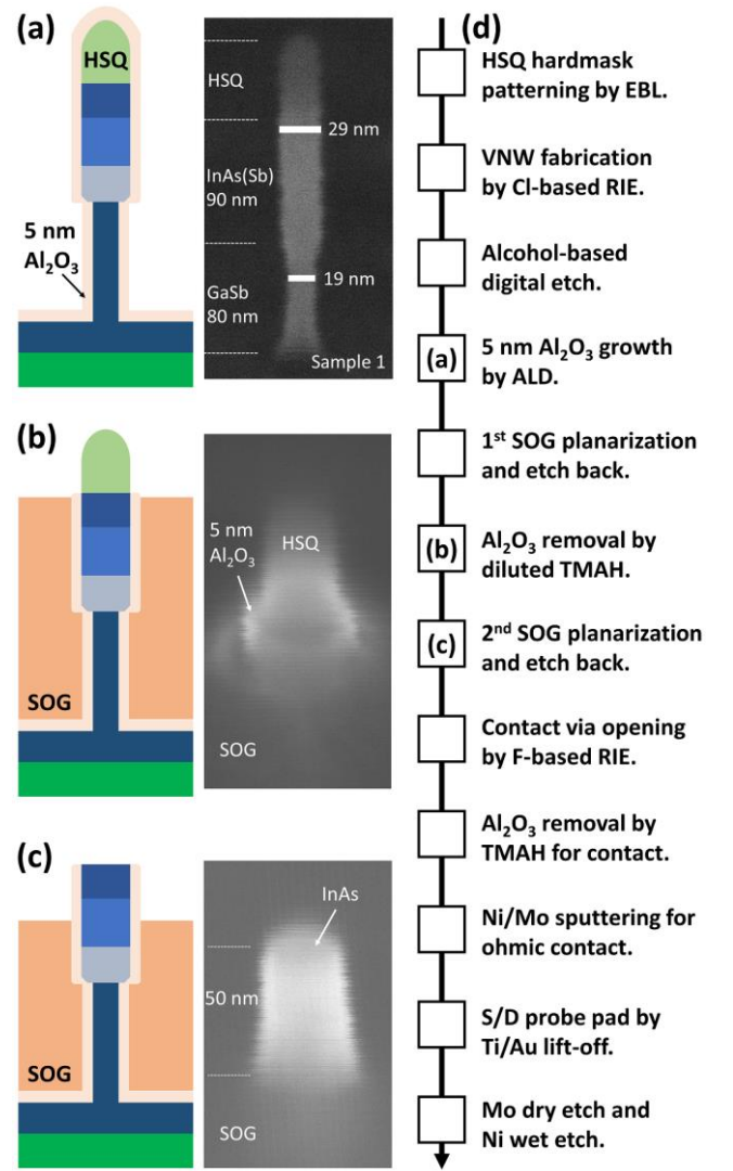
Fig. 2. Schematics of key processing steps and process flow. Schematics and corresponding SEM images after ALD Al 2 O 3 growth (a); after 1 st SOG planarization, etch back and Al 2 O 3 removal (b); after 2 nd SOG planarization and etch back (c). (d) Process flow for GaSb/InAs(Sb) VNW Esaki diode fabrication.
