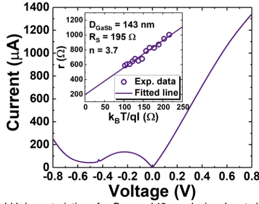
Fig. 6. I - V characteristics of a D_{\text{GaSb}} = 143 nm device. Inset shows the linear regression between differential resistance and k_B T / q l , through which series resistance and ideality factor are extracted.
