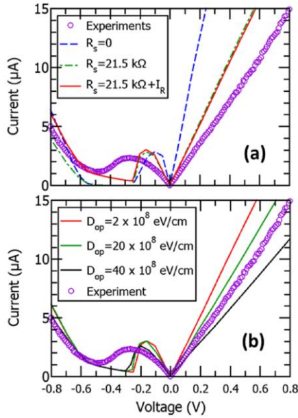
Fig. 9. Simulated (lines) and experimental (symbols) I - V curves for the D_{\text{GaSb}} = 11 nm device. (a) Simulations with and without experimentally estimated R_s and fitted I_R . (b) Simulations including R_s , I_R as in (a) and inelastic polar optical phonon scattering for different deformation potential ( D_{\text{op}} ) values.
