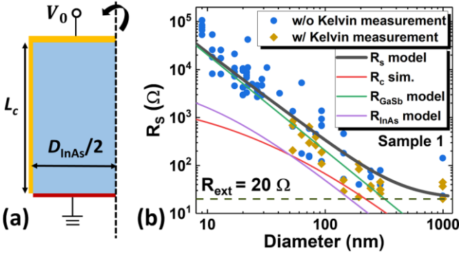
Fig. 7. (a) Radial cross section of the \text{Ni}/n^+-\text{InAs} top contact for R_c TCAD simulations. Yellow and red edges denote the top contact, with an applied voltage of V_0 , and ground, respectively. (b) R_s versus GaSb diameter for extracted R_s from experimental results from sample 1 (dots) and for modeled R_s (black line). Different components of R_s including R_c , R_{\text{GaSb}} , R_{\text{InAs}} , and R_{\text{ext}} are also shown.
