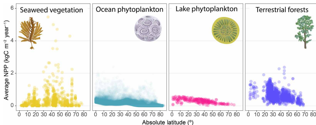
Fig. 4. Relationship between latitude and NPP across Earth's major primary producers. Lines depict the smoothed modeled mean. Terrestrial forest NPP includes above- and belowground productivity.
