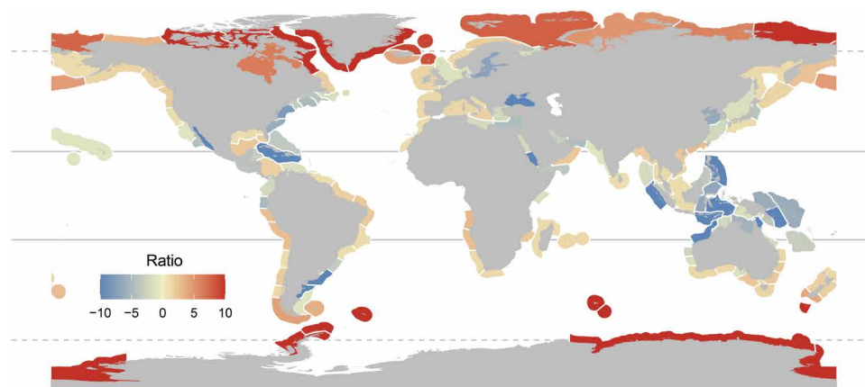
Fig. 3. Relationship between subtidal seaweed forest and coastal phytoplankton productivity ( \text{gC m}^{-2} \text{ year}^{-1} ) across the world's marine ecoregions. The ratio indicates the relative magnitude between subtidal seaweed forest and coastal phytoplankton per-area NPP, with positive ratios indicating seaweed forest NPP being greater. The ratio of ecoregions where NPP of marine forests or phytoplankton was not available is not shown. Lines indicate the tropics and polar circles.
