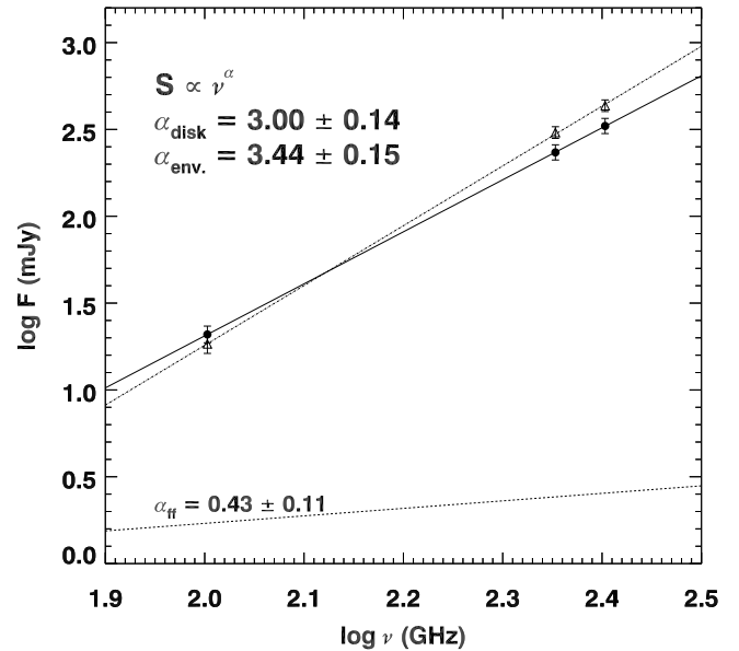
Fig. 4. Spectral energy distribution determined for the dust emission within the circumbinary disc ( \alpha = 3.0 , black line) and in the envelope ( \alpha = 3.4 , dotted dashed line). The flux densities for the disc and envelope are indicated as filled circles and open triangles, respectively. The errors are dominated by the uncertainty in the flux calibration, which is assumed to be \sim 10\% . The dashed line shows the SED determined from the free-free (centimetric) emission detected with the Very Large Array ( Alves et al. 2019 ).
