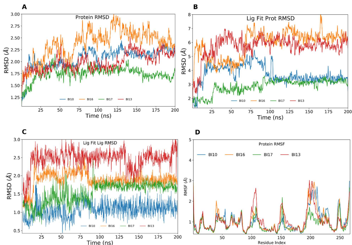
Fig. 9. MD simulations of the complexes formed between InhA and the four hit compounds. (A) RMSD graph of InhA Cα atoms across 200 ns MD simulations. (B) LigFitProt RMSD graph. (C) LigFitLig RMSD graph. (D) RMSF graphs.
