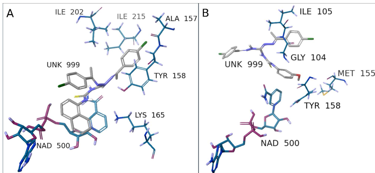
Fig. 6. . 3D interaction diagram of BI-17 (A) and BI-16 (B) within the active site of InhA.
