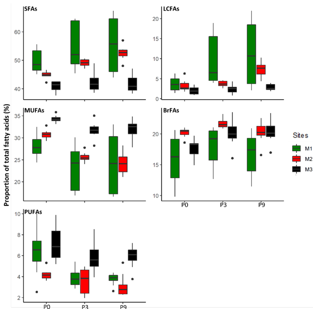
364 365 Figure 7: Contribution (% of total fatty acids) of SFAs, LCFAs, MUFAs, BrFAs and PUFAs to the 366 total fatty acid pool in the sediments of the three mangroves (M1 in Ilha Grande Bay, M2 in 367 Guanabara Bay and M3 in Sepetiba Bay.). Median values (horizontal solid line inside the box), 25th 368 and 75th percentiles (lower and upper ends of the boxes), 95% confidence intervals (whiskers) and 369 outliers (circles) are shown. (1 column)
