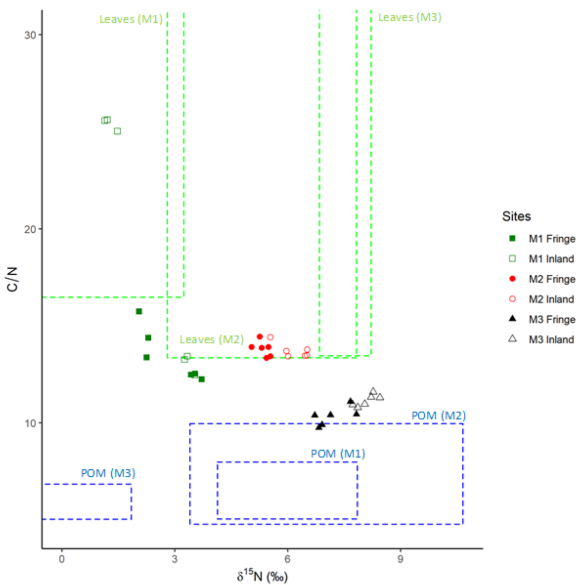
274 275 Figure 4: Plot of \delta^{15}\text{N} vs C/N in sediments mangroves of the three mangroves sites -: M1 in Ilha 276 Grande Bay, M2 in Guanabara Bay and M3 in Sepetiba Bay. The envelopes of leaves are 277 represented by green boxes and those of particulate organic matter in water are represented by 278 blue boxes. (1 column)
