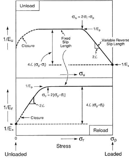
Figure 15: Evolution of the tangent compliance during a unidirectional unloading-reloading cycle during matrix cracking for a unidirectional composite, extracted from [27].
