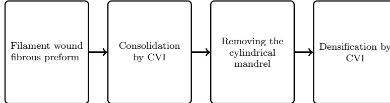
Figure 1: Different stages in the development of a CVI-SiC/SiC composite.
