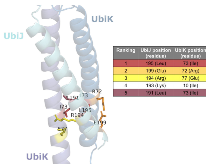
Figure 5. Co-evolution analysis. The top 5 best co-evolved residue pairs are listed in the table on the right and mapped onto the 3D structure of the heterotrimer on the left.
