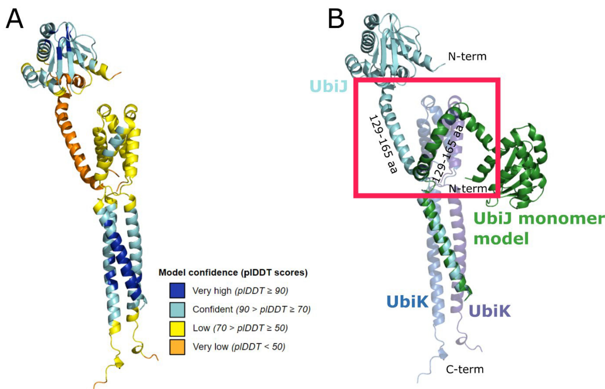
Figure 4. Modelling of the heterotrimer (UbiJ-UbiK 2 ). (A) Heterotrimer prediction using AF2 coloured according to the pLDDT score and shown in cartoon. (B) Structural superimposition of the best AF2 model and the UbiJ monomer, shown in green cartoon.
