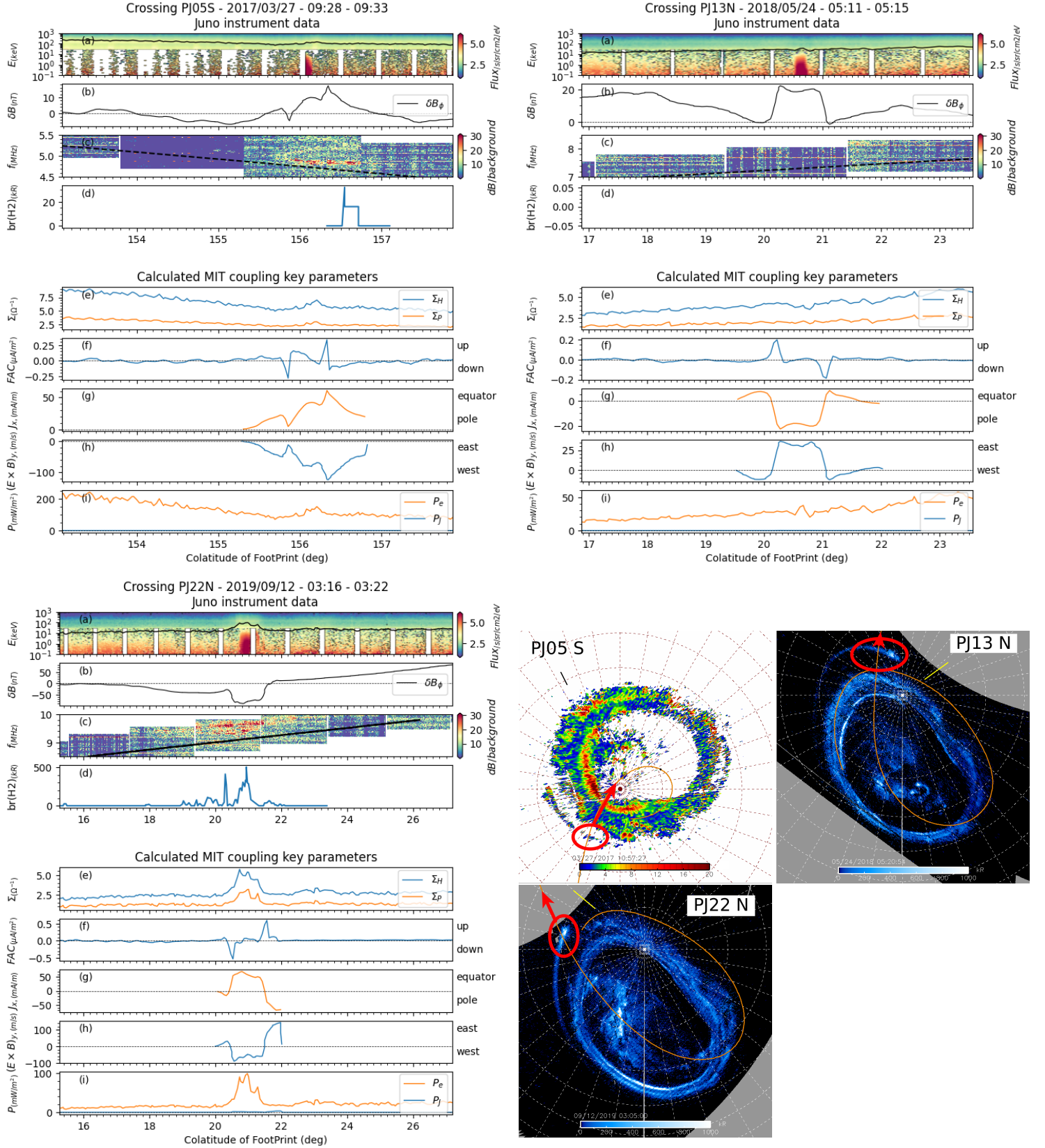
Figure 5: Same as figure 3, but for Io's tail flux tube crossings. UVS imagery for perijove 5 is shown in units of color ratio rather than in kR to enhance the visibility of the crossing between the trajectory of Juno's footprint and Io's tail.
