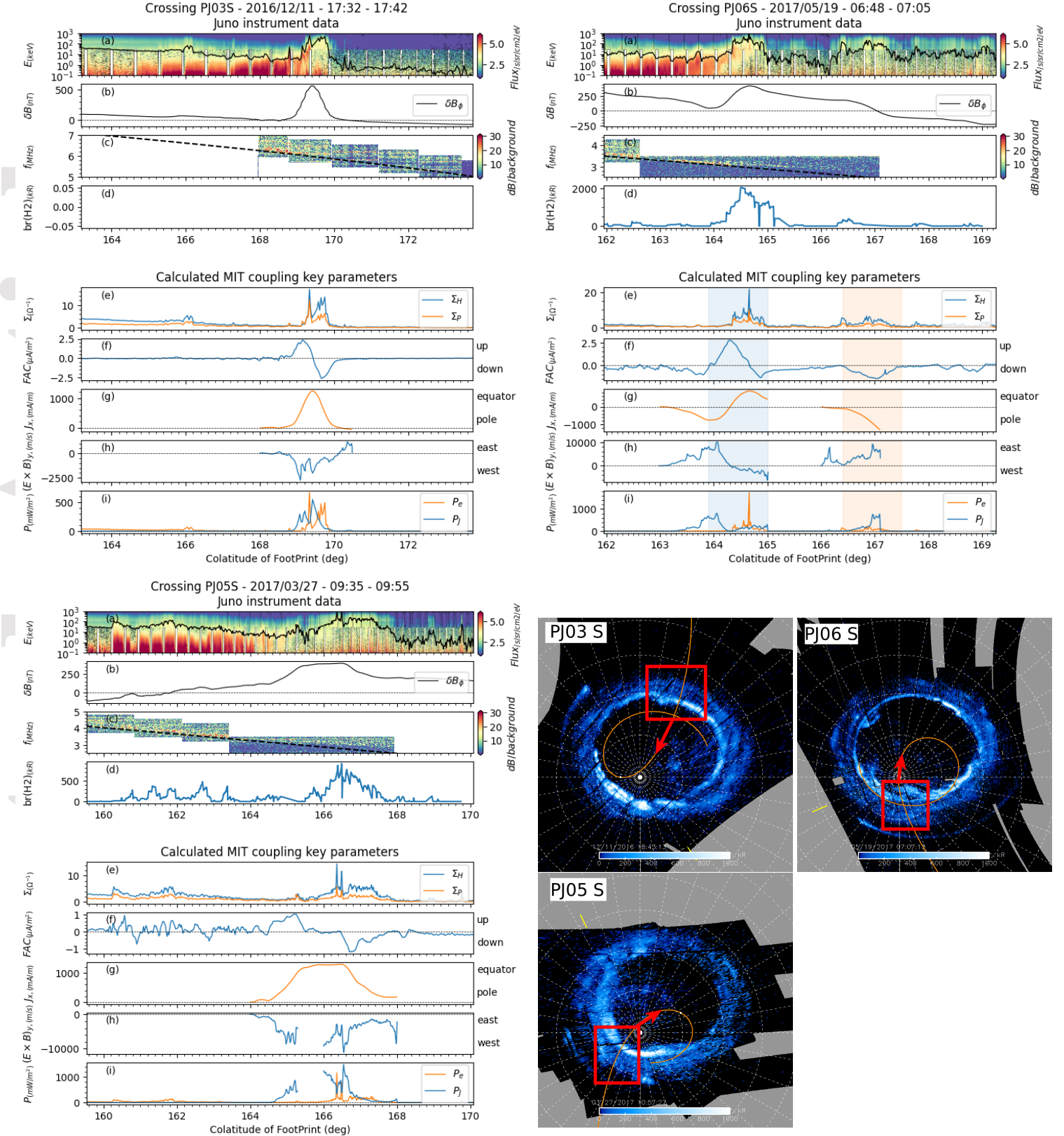
Figure 3: Juno instrument data (top four rows of each panel) and MIT key parameters calculated from them (bottom five rows of each panel) plotted as a function of the magnetic co-latitude of Juno's magnetic footprint for southern perijoves PJ03 (top left panel), PJ06 (top right panel) and PJ05 (bottom left panel). For each of these crossings, the corresponding UVS maps are shown at the bottom right of the figure.
