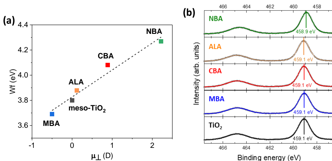
Figure 3. (a) UPS-derived work function W_f of the different SAMs adsorbed onto TiO 2 plotted against the calculated normal dipole moment \mu_{\perp} . (b) XPS core level signals of Ti 2p. The data (open circles) is fitted by two Voigt profiles (colored line) corresponding to the 2p 1/2 and 2p 3/2 Signal. The position of the latter one is indicated in the graph and listed in Table 1 as E_{B, TiO_2} .
