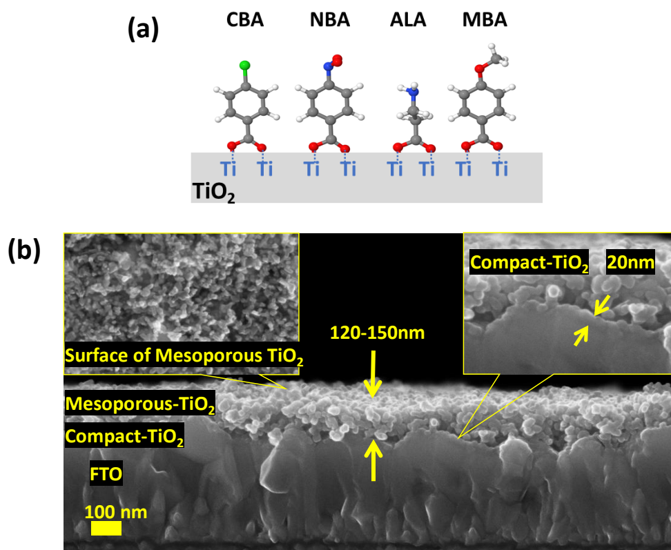
Figure 1: (a) Schematic molecular structure of the studied SAMs bonded to the anatase TiO 2 surface. From left to right: 4-chlorobenzoic acid, 4-nitro benzoic acid, \beta -alanine and 4-methoxy benzoic acid. White ball: hydrogen, grey: carbon, red: oxygen, blue: nitrogen and green: chlorine. (b) Cross-sectional SEM view of Glass/FTO/ c -TiO 2 / meso -TiO 2 /SAMs. The left inset shows the morphology of meso -TiO 2 surface, and the right inset is a zoom view of the c -TiO 2 layer cross-section.
