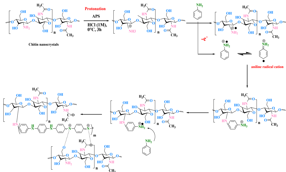
Figure 3. Mechanism of PANI synthesis and grafting onto ChNCs.
