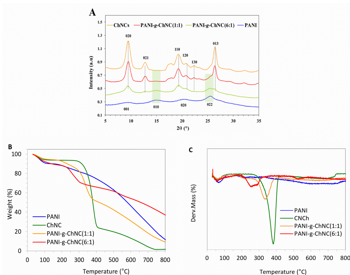
Figure 4. XRD patterns of ChNCs, PANI and PANI-g-ChNCs (A), TG (B) and DTG (C) curves of pure PANI, ChNCs and PANI-g-ChNCs.
