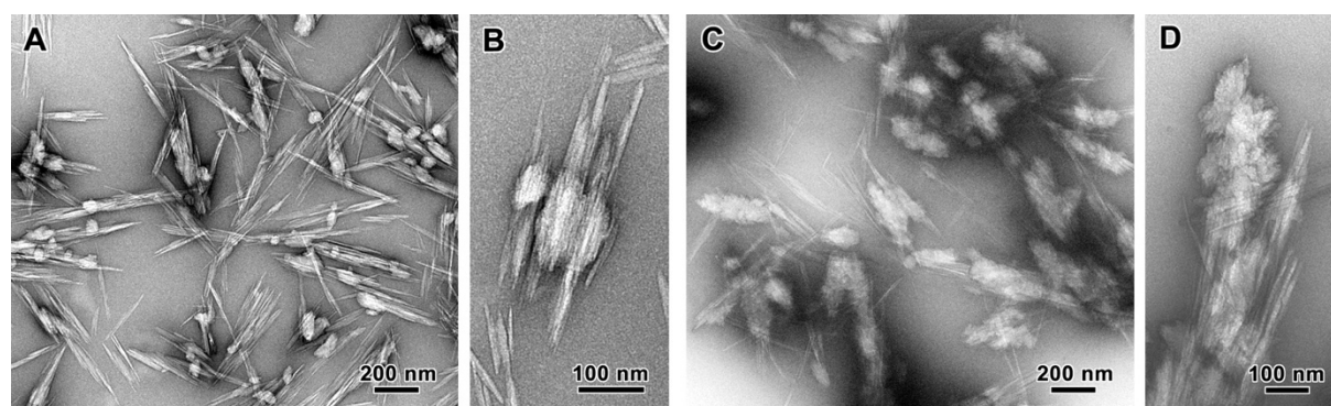
Figure 2. A-D) TEM images of negatively stained preparations of neat PANI-g-ChNC (1:1) (A,B) and PANI-g-ChNC (6:1) (C,D).
