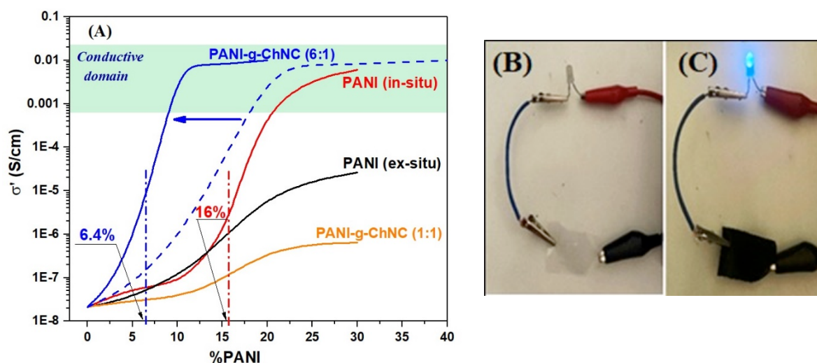
Figure 8. (A) DC electrical conductivity of PANI/PVA films using simple mixing (SM) and in-situ polymerization (ISP) and PANI-g-ChNC/PVA nanocomposites as a function of PANI content. Demonstration of the conductivity through a LED lamp: neat PVA matrix (B) and PANI-g-ChNC/PVA (C).
