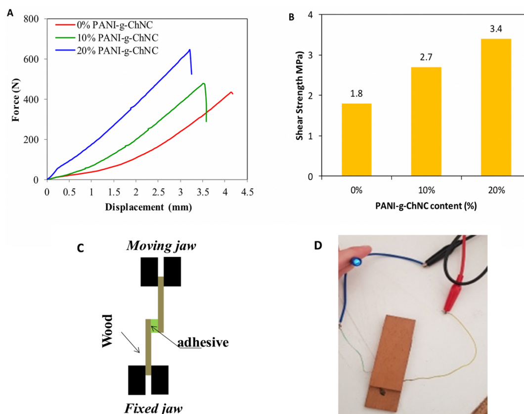
Figure 9. (A) Force vs. displacement during tensile shear test for the wood joint, and (B) shear strength at different content of PANI-g-ChNCs (6:1) for wood joints bound with PVA-based adhesive containing different amounts of PANI-g-ChNCs (6:1). (C) Schematic representation of the shear test specimen, and (D) conductivity demonstration of the adhesive containing 20 wt% PANI-g-ChNCs.
