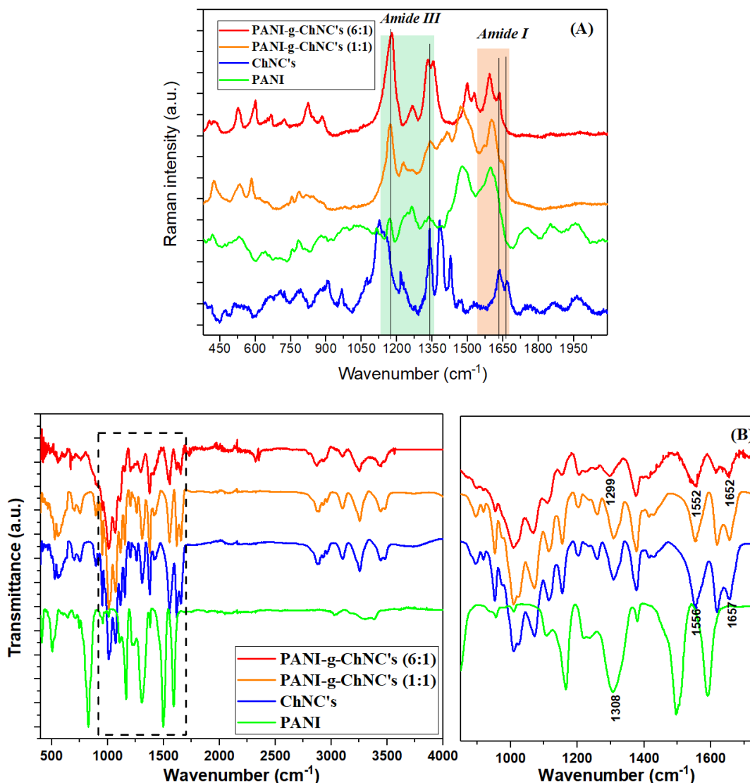
Figure 5. Raman spectra (A) and FTIR spectra (B) of ChNCs, PANI, and PANI-g-ChNCs.
