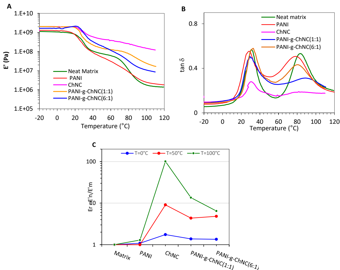
Figure 6. (A) Variation of storage modulus E' and (B) \tan \delta with temperature for neat PVAc matrix and nanocomposite films containing 13 wt% of PANI, ChNCs, PANI-g-ChNCs (1:1) and (6:1); (C) plot of E_r vs. nanofiller type at 50 and 100 °C.
