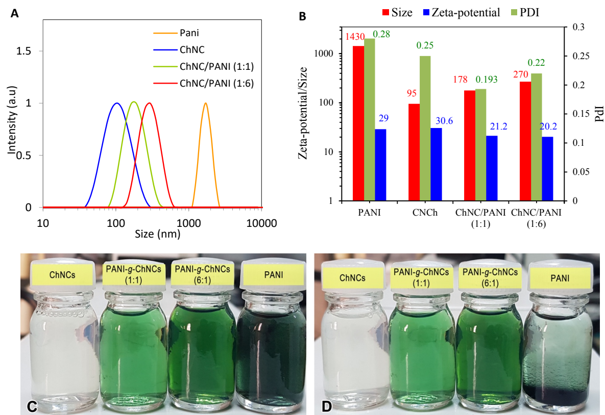
Figure 1. Particle size distribution (A) and \zeta -potential/mean-particle size/polydispersity index (B) of ChNC, PANI, PANI-g-ChNC (1:1) and PANI-g-ChNC (6:1) suspensions prepared by in-situ polymerization; C,D) Photos of the ChNC, PANI, PANI-g-ChNC (1:1) and PANI-g-ChNC (6:1) suspensions after a 10-s sonication (C) and a 24-h standing (D).
