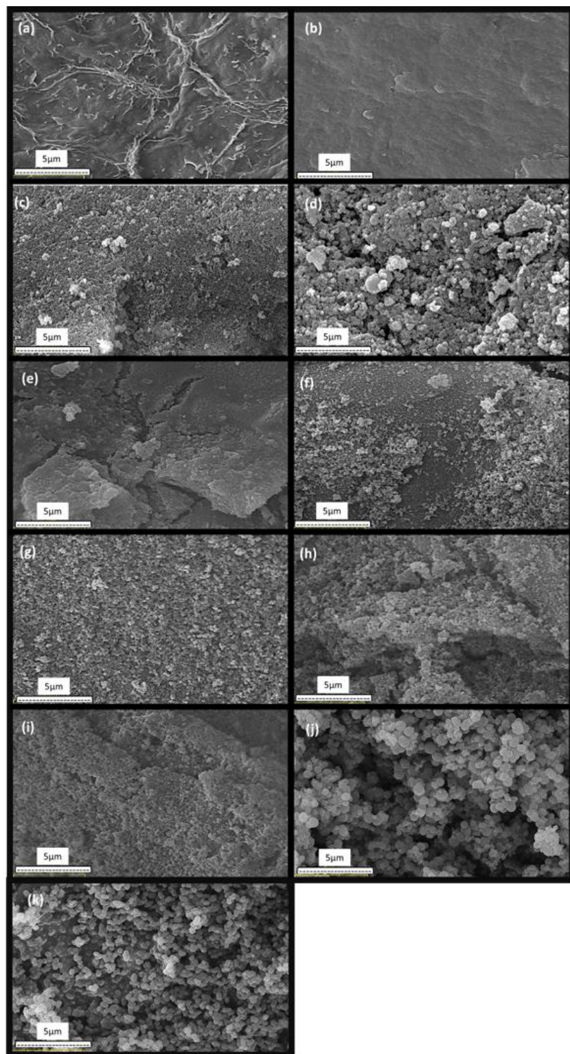
Figure 5 - SEM images of (a) ST-M1, (b) ST-M2,(c) SSMMP-M1, (d) SSMMP-M2 (e) SSMMP-20%-Im(Me)-NTf 2 , (f) SSMMP-10%-Im(Me)-NTf 2 , (g) SSMMP-5%-Im(Me)-NTf 2 , (h) SSMMP-5%-Im(nBu)-I, (i) SSMMP-5%-Im(nBu)-NTf 2 , (j) MCM-41 and (k) MCM-48
