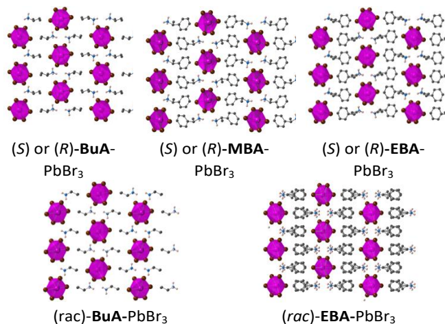
Figure 3: Representation of the structures of either ( S )- or ( R )- BuA-PbBr 3 , MBA-PbBr 3 , EBA-PbBr 3 , ( rac )- BuA-PbBr 3 and ( rac )- EBA-PbBr 3 , projection in the xOz planes. Only H atoms located on N are presented. For bond and distances see text.
