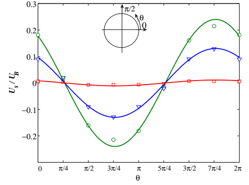
FIG. 3: Azimuthal variation of the streak velocity at Re = 2420 , r/R = 0.72 and at the three axial positions: z = 20D (square), z = 54D (nabla) and z = 122D (circle).
