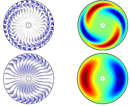
FIG. 1: Cross-flow in the (r - \theta) section and optimal streaks at Re = 2420 , n = 0.5 and a = 0.1 . (Top): Optimal perturbation with m = 2 and \alpha = 1.20 ; (bottom) stream-wise independent vortices with m = 1 . The red and blue zones correspond respectively to the fast and low streaks
