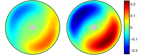
FIG. 4: Cross-section in (r, \theta) at two axial positions z/D = 54 and 122 show contours of iso- (U - \bar{U})/U_B , with the fast streaks (red/dark bottom) and low streaks (blue/dark top). Re = 2420 , n = 0.5 and a = 0.1 .
