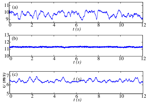
FIG. 5: Instantaneous axial velocity plots at Re = 2420 , z = 122D , n = 0.5 and r_0/R = 0.1 . (a) r/R = 0.72 , \theta = 7\pi/4 ; (b) r/R = 0 and (c) r/R = 0.72 , \theta = 3\pi/4 .
