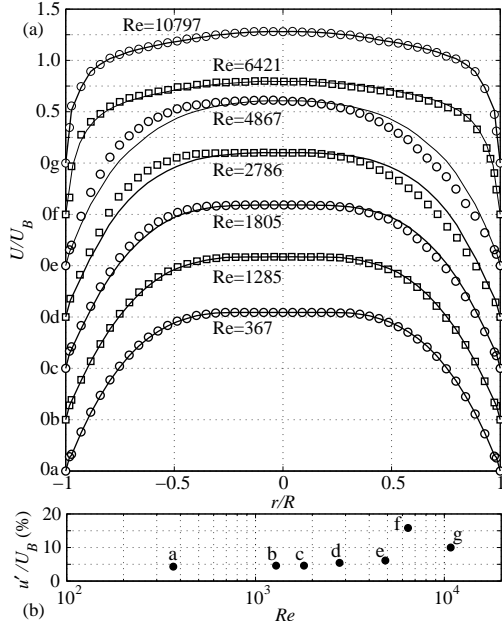
FIG. 2: (a) Mean axial velocity profiles at different Reynolds number, \tau_0 = 9.75 Pa, K = 3.82 Pa.s n , n = 0.47 ; (b) Axial velocity fluctuations level u'(rms)/U_B vs Re at r/R = 0.8 .
