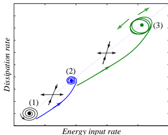
FIG. 6: Qualitative description of the transition process in the phase diagram displaying dissipation rate versus energy input rate. Point (1) is the steady, one-dimensional laminar state, towards which, the system returns spirally when Re < Re_{c1} . Point (2) is the non-linear stable asymmetric state. Node (3) represents the fully developed turbulent regime. The crosses with arrows sketch unstable saddle nodes. Flow trajectories are sketched for increasing values of Re .
