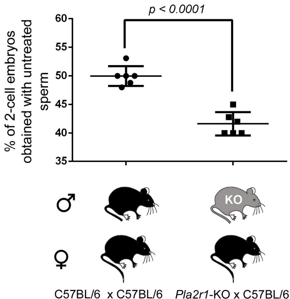
Figure 8. IVF outcome is decreased when sperm were obtained from Pla2r1 -KO males. Comparison of the % of two-cell embryos generated by IVF, using oocytes from C57BL/6 and sperm from either WT or Pla2r1 -KO littermate males ( n = 6 for KO and WT males). n represents the number of biological replicates, and the statistical difference was assessed using the t -test and p -value, as indicated.
