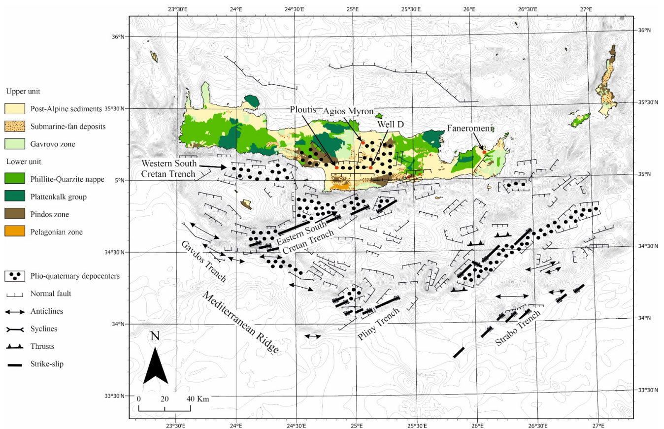
Figure 2. Scheme illustrating the tectonic zonation and main structural elements and depocenters of Crete Island and surrounding regions. Red cycles correspond to the sampling locations.
