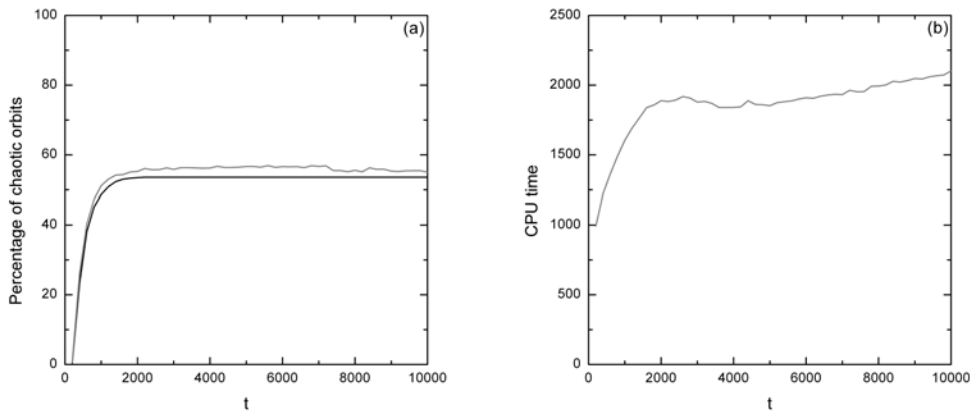
Figure 3. (a): The percentage of the chaotic orbits (having SALI < 10^{-8} ) with initial conditions on the PSS of Hamiltonian (2) for E = 1/8 as a function of the integration time t . (b): The evolution of the CPU time (in sec) needed for the fast scanning of the PSS. In panel (a) black line corresponds to the full scanning of the PSS while grey lines of both panels to the fast PSS scanning.
