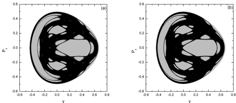
Figure 2. Regions of different values of the SALI on the PSS x=0 of the Hénon-Heiles system (2) for a grid of 500 \times 500 equally spaced initial conditions. In (a) the SALI was computed for every initial condition (full PSS scanning) while in (b) the final value of the SALI is attributed not only to the initial condition but also to all successive intersection points of the orbits with the PSS.
