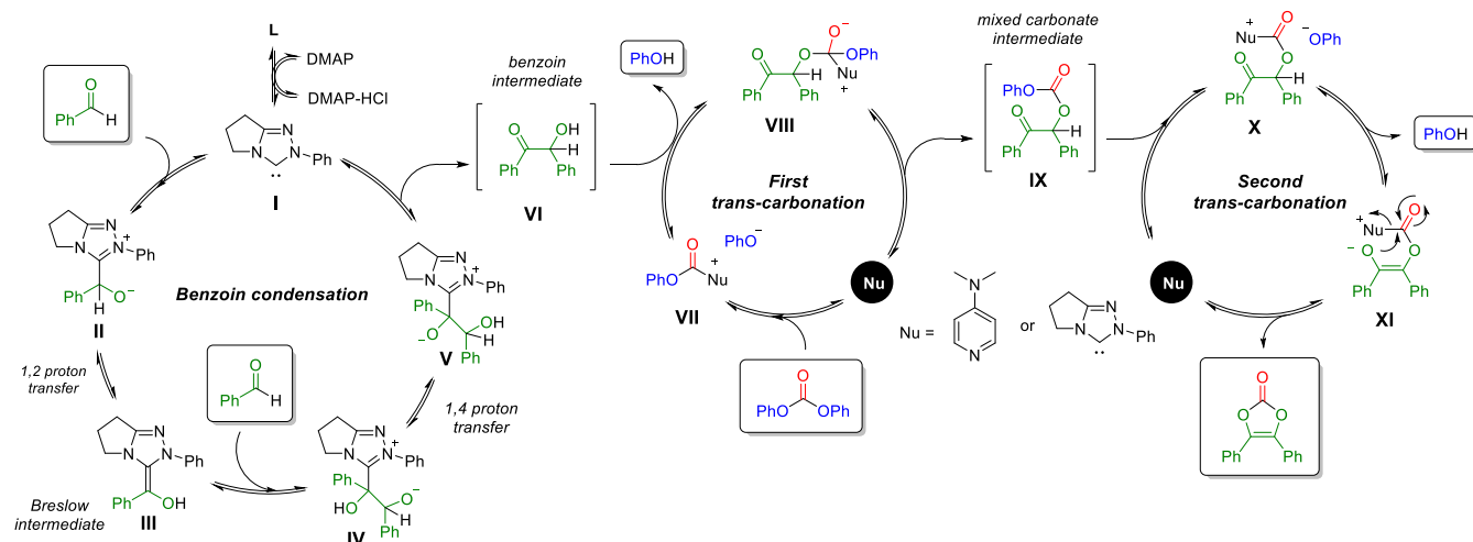
Scheme 6. Mechanism proposal.
