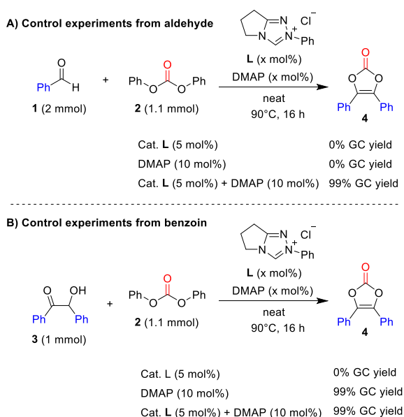
Scheme 5. Control experiments.
