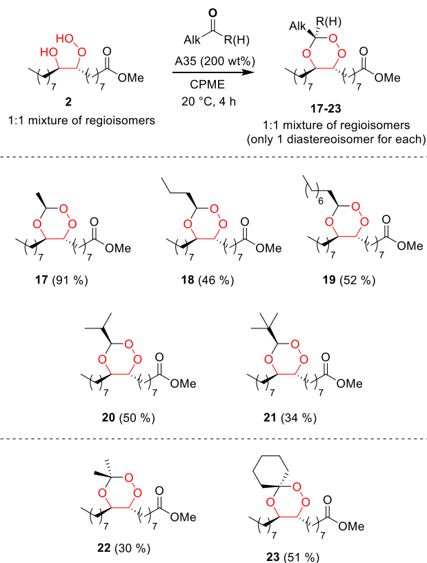
Figure 2. Preparation of 1,2,4-trioxanes from \beta -hydroxy hydroperoxide 2 and a range of aliphatic aldehydes and ketones.
