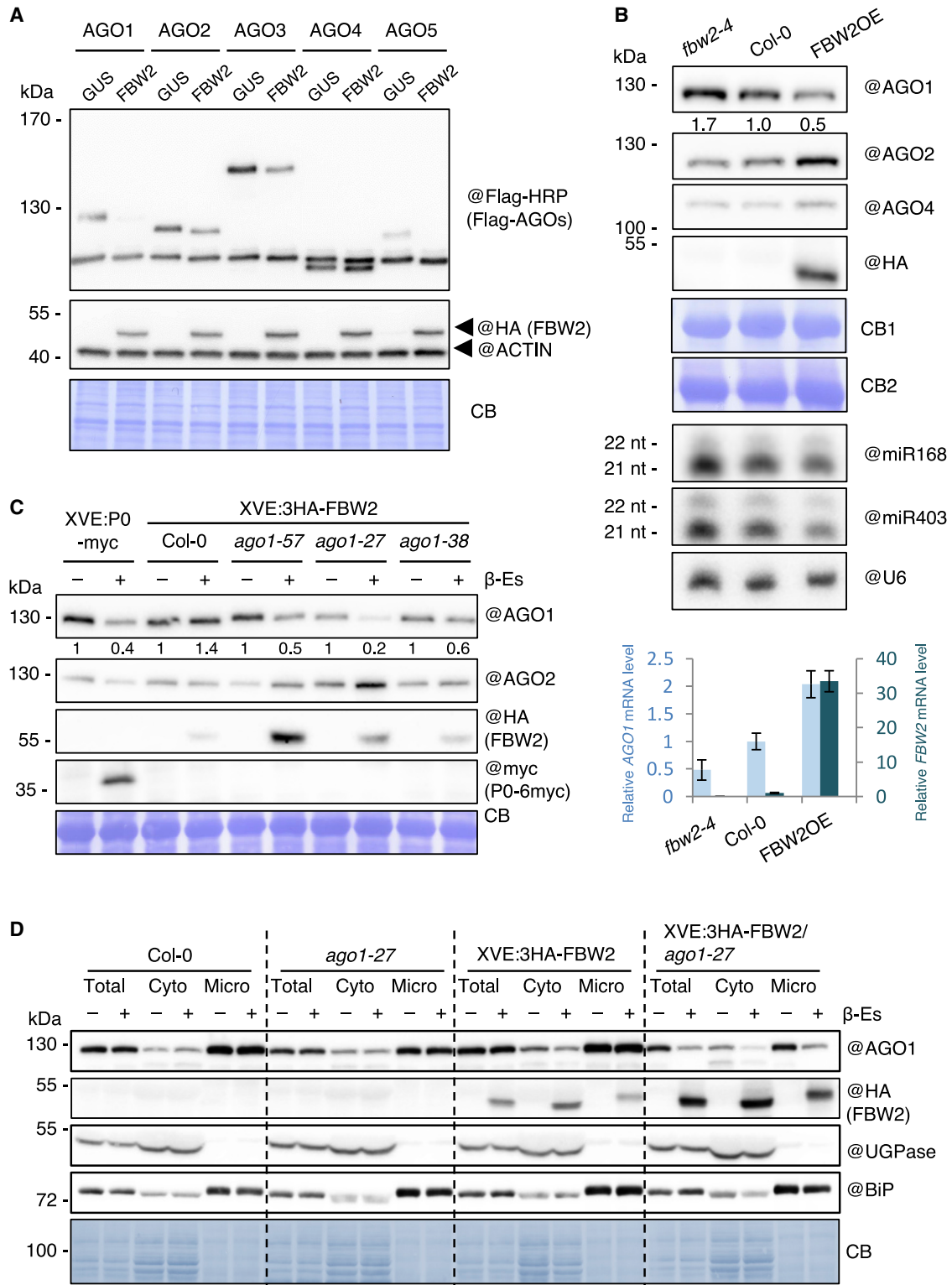
Figure 1. FBW2 triggers preferential degradation of AGO1
